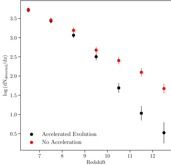
Figure 26. Predicted total number of galaxies as a function of redshift in the full JADES area detected at \gtrsim 5\sigma . We plot results from the mock with the accelerated evolution above z = 8 with black points against those with the evolution predicted by Bouwens et al. (2015) with red points. The uncertainties include both Poisson error, and cosmic variance estimated from the Trenti & Stiavelli (2008) “cosmic variance calculator”. Data from the JWST GTO program will help to discern between the two evolutionary scenarios at high redshift.
