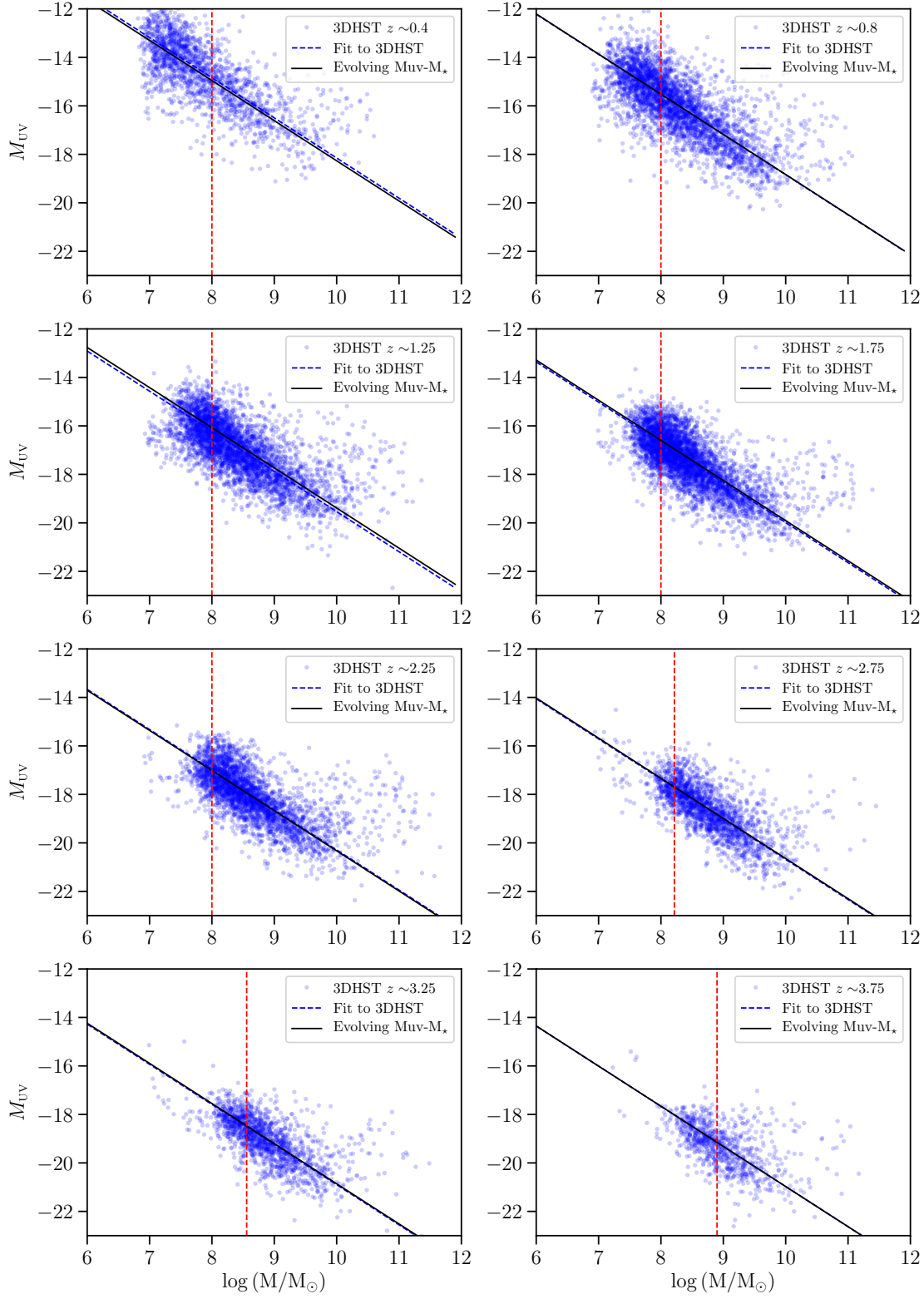
Figure 6. The M_{UV}-M_* relation for realizations of the SED-fitting of observed star-forming galaxies ( \log(\text{sSFR}) < -10 \text{ Gyr}^{-1} ) in the 3DHST survey (blue points) with high-confidence measurements of M_{UV} , M , and redshift as described in Sections 3.2 and 3.4.1. Blue dashed lines indicate the best-fitting linear relationship under the assumption of a fixed slope as described in the text. Solid black lines indicate the smoothly evolving redshift-evolution of the M_{UV}-M_* relation in our model as characterized in Figure 7 and Equation 11. The red dashed line indicates the stellar mass above which mock galaxies are matched to 3D-HST realizations, which is the larger between \log(M/M_\odot) > 8 and \log(M/M_\odot) > 6.3 + 0.7z (the evolving mass limit exceeds \log(M/M_\odot) > 8 at z > 2.4 ).
