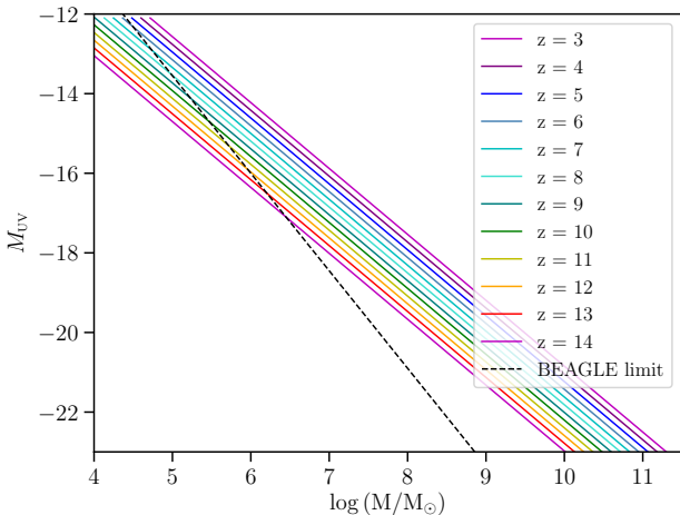
Figure 8. Demonstration of the evolution of the mean M_{\text{UV}}-M_* relation with redshift, (if mass to light ratios were allowed to continue decreasing above z > 8 ), in comparison to the mass-to-light ratio limit imposed by the stellar population modeling with BEAGLE (which implicitly assumes a Chabrier IMF with a high mass cut-off of 100 M_\odot .) In our model, all z > 8 galaxies follow the M_{\text{UV}}-M_* relation at z = 8 to avoid a scenario where significant numbers of galaxies exceed the theoretical mass-to-light ratio limit set by BEAGLE.
