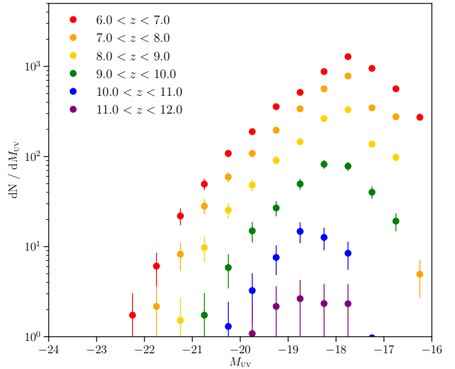
Figure 25. Predicted total number of objects detected as a function of M_{UV} in bins of redshift for JADES. Objects are selected as “detected” if they are brighter than the 5\sigma limits in two photometric bands corresponding to the rest-frame UV, similar to common LBG selection techniques.
