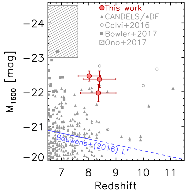
Figure 5. Distribution with redshift of the absolute magnitude of the bright LBGs detected so far at z \gtrsim 7 . We include measurements of Oesch et al. (2014); Bouwens et al. (2015); Roberts-Borsani et al. (2016); Calvi et al. (2016); Bowler et al. (2017) and Ono et al. (2017) as indicated by the legend. Our candidate LBGs are marked as red points with error bars and lie at the high luminosity end of all candidate z \sim 8 LBGs to date. Given the depth and wavelength coverage of the observations available for our sources, our bright sample arguably constitutes the brightest and most reliable sample of z \sim 8 - 9 galaxies to date.
