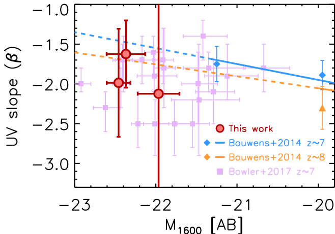
Figure 6. Rest-frame UV continuum slope ( \beta ) versus UV absolute magnitude for the three z \gtrsim 8 LBGs (red points with errorbars). Individual measurements for the sample of z \sim 7 LBGs of Bowler et al. (2017) are indicated by the purple points. The blue and yellow points mark the bi-weight median measurements of Bouwens et al. (2014) for the z \sim 7 and z \sim 8 samples, respectively. The corresponding best fit relation is shown by the solid blue and yellow lines. The dashed lines indicate the extrapolations of these relations to the luminosities probed in this work. Our measurements of \beta are consistent with the extrapolations of the z \sim 7 - 8 relations.
