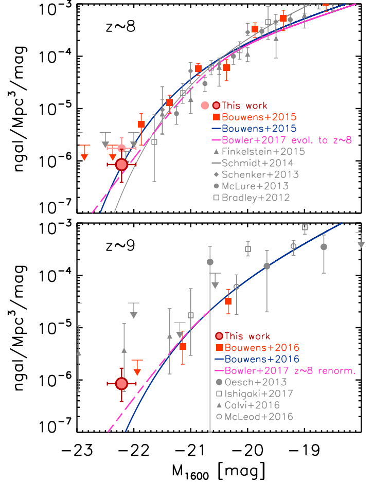
Figure 9. Top panel: The red point with errorbars marks our estimate of volume density associated to the sample of candidate luminous z \gtrsim 8 galaxies considered in this work. The pink filled circle corresponds to the volume density after adding to the sample three luminous z \sim 8 LBGs from Labbé et al. (2017, in preparation), not targeted in the HST proposal. Recent UV LF determinations at z \sim 8 from Bradley et al. (2012); McLure et al. (2013); Schenker et al. (2013); Schmidt et al. (2014); Bouwens et al. (2015); Finkelstein et al. (2015) are also reported, with plotting conventions detailed by the legend. The blue curve corresponds to the Schechter form of Bouwens et al. (2015), while the magenta curve represents the evolution to z \sim 8 of the z \sim 7 DPL of Bowler et al. (2017) according to Bouwens et al. (2016b). Bottom panel: Here we compare our volume density estimate (red point) to measurements of the UV LF at z \sim 9 (Oesch et al. 2013; Bouwens et al. 2016b; Calvi et al. 2016; McLeod et al. 2016; Ishigaki et al. 2017). The blue curve represents the Schechter function from Bouwens et al. (2016b). The magenta curve presents the bright-end of the dual power law from Bowler et al. (2017) evolved to z \sim 8 following Bouwens et al. (2016b) whose characteristic density has been adjusted to match that of the Schechter function at the characteristic luminosity.
