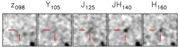
Figure 2. Image stamps, in inverted grey scale, centered at the position of UVISTA-Y-1, in the five HST bands available for this object, i.e. the three canonical bands targeted by our HST program (PI: R. Bouwens - z_{098} , J_{125} and H_{160} ) plus Y_{105} and JH_{140} from the SUSHI program (PI: N. Suzuki). The source is clearly detected in the J_{125} , JH_{140} and H_{160} bands, while it is only slightly detected ( 2.2\sigma ) in Y_{105} . The cutouts in the HST /WFC3 bands have been smoothed with a \sigma = 1.4 pixels gaussian kernel.
