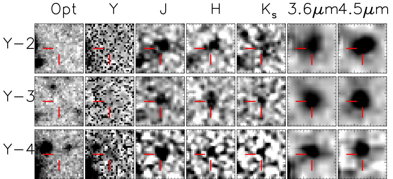
Figure 10. Image stamps in inverted grey scale of the three additional bright candidate z \gtrsim 8 LBGs in the stacked optical, stacked Y, UltraVISTA J , H and K_S and Spitzer IRAC 3.6\mu\text{m} and 4.5\mu\text{m} bands. Each row corresponds to a source, as labeled on the left, where we omitted the prefix UVISTA- from the object name for clarity. Each cutout is 5''.0 \times 5''.0 .
