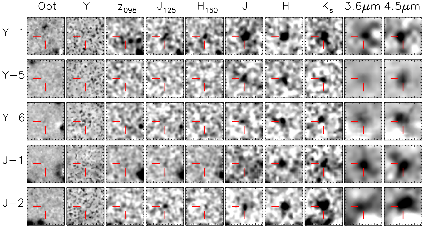
Figure 1. Image stamps in inverted grey scale of the five bright candidate z \gtrsim 8 LBGs in the stacked optical, stacked Y , HST /WFC3 z_{098} , J_{125} , H_{160} , UltraVISTA J , H and K_S and Spitzer IRAC 3.6\mu\text{m} and 4.5\mu\text{m} bands. Each row corresponds to a source, as labeled on the left, where we omitted the prefix UVISTA- from the object name for clarity. Each cutout is 5''.0 \times 5''.0 . The ground based and IRAC cutouts are shown after removing the neighbours. The cutouts in the HST /WFC3 bands have been smoothed with a \sigma = 1.4 pixels gaussian kernel. Postage stamp images of three other ultra-luminous ( M_{UV} \lesssim -22 ) z \sim 8 candidates are presented in Figure 10 from Appendix B.
