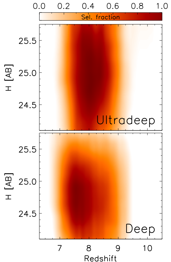
Figure 8. Selection functions corresponding to the criteria adopted to identify candidate z \sim 8 LBGs, computed with a Monte Carlo simulation on real data. The top panel refers to the ultra-deep stripes, while the lower panel to the UltraVISTA deep stripes. The original un-evenly spaced measurements have been smoothed with a boxcar filter of 5 pixels, after casting them onto a regular grid for display purposes. Darker regions correspond to higher selection rates as indicated by the scale at the top of the figure. Our criteria allow us to select galaxies at 7.1 \lesssim z \lesssim 9.2 and 6.9 \lesssim z \lesssim 9.3 , respectively for the ultra-deep and deep regions.
