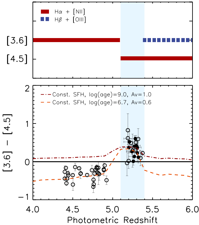
Figure 2. Nebular emission line contamination in the 3.6 and 4.5 \mu m photometric filters. Top panel: the redshift ranges over which the dominant nebular emission lines, H \alpha , H \beta , [O III], [N II], and [S II], contribute to the 3.6 and 4.5 \mu m flux measurements. Lower panel: the predicted [3.6]–[4.5] colour due to various nebular emission lines as a function of redshift. The solid black circles indicate sources that are selected in the redshift range z_{\text{phot}} = 5.1-5.4 , where H \alpha lies in the 4.5 \mu m filter, while 3.6 \mu m is devoid of strong nebular emission. Their observed [3.6]–[4.5] colours are primarily very red. The open circles are the colours for the spectroscopic sample found in Vanzella et al. (2009), which we use to estimate a stellar continuum colour of \sim 0.00 mag. The dashed and dot-dashed lines indicate two different models from the stellar population synthesis code BPASS (Eldridge & Stanway 2012). While a galaxy with modest emission lines (rest-frame H \alpha + [N II]+[S II] EW \sim 190 Å) and significant reddening (dot-dashed line; age = 10^9 yr, A_V = 1.0 ) can reproduce the z \sim 5.2 galaxy colours, the model does not reproduce the z < 5 galaxy colours. A young galaxy with strong emission lines (rest-frame H \alpha + [N II]+[S II] EW \sim 580 Å) and lower dust content reproduces both galaxy colour distributions at z < 5 and \sim 5.2 (dashed line; age = 10^{6.7} yr, A_V = 0.6 ).
