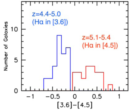
Figure 3. [3.6]–[4.5] colour distribution for sources in our z = 5.1 – 5.4 primary selection (red histogram) and z = 4.4 – 5.0 control sample (blue histogram: Appendix A). Sources where H \alpha + [N II] is in the [3.6] band uniformly have moderately blue colours, whereas sources with H \alpha + [N II] in the [4.5] band uniformly have moderately red colours. The impact of the H \alpha + [N II] emission lines on the IRAC [3.6]–[4.5] colour is quite clear. Deriving the H \alpha + [N II]+[S II] EW by contrasting the observed [3.6]–[4.5] colour of sources in the two samples should produce a very robust result.
