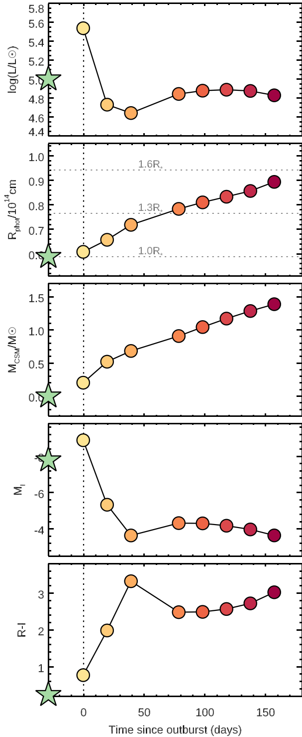
Figure 5. Evolution of the star’s observables during the outburst. Top panel: bolometric luminosity; second top panel: the radius of the photosphere, defined as the flux-weighted average of the R_{\lambda}(\tau = 1) surface; centre panel: circumstellar mass, defined as the mass now above the original photosphere; second bottom panel: absolute magnitude in the I -band; bottom panel: R - I colour. The green star indicates the properties of the base model. The vertical dashed line indicates the time at which the subsurface eruption breaks the surface of the star, defined in M20 as t = 140 d, but defined here as t = 0 .
