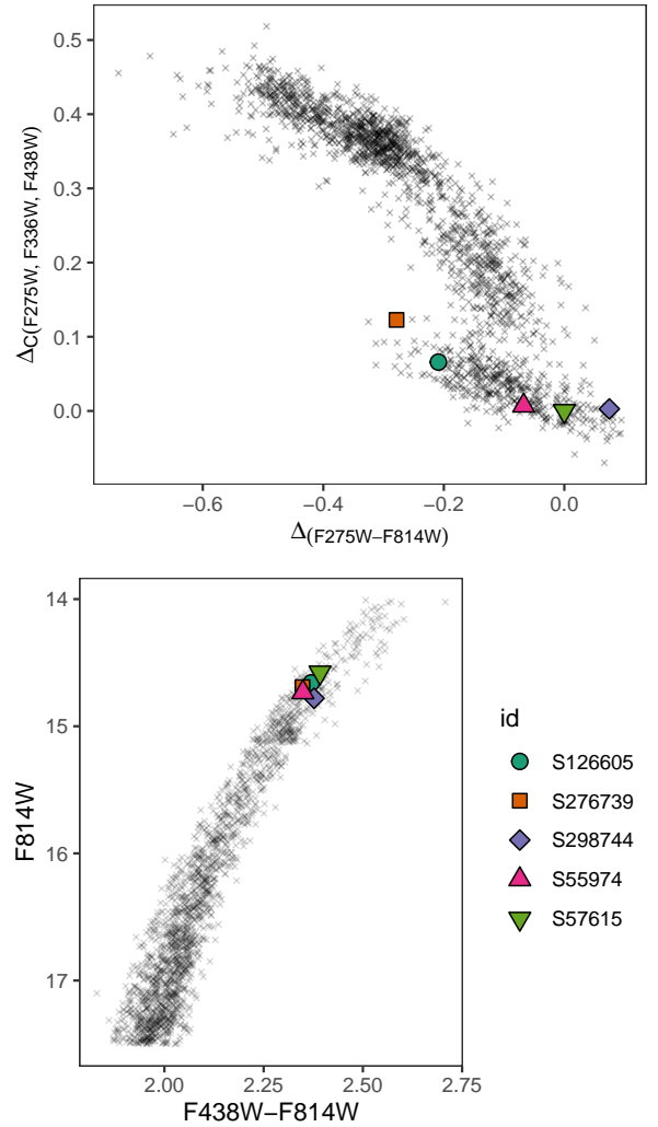
Fig. 1. Positions of the target stars in the chromosome map and in the F814W-(F438W-F814W) CMD of NGC 2808 are shown in the top and bottom panel, respectively. Photometric data are from Nardiello et al. (2019).
