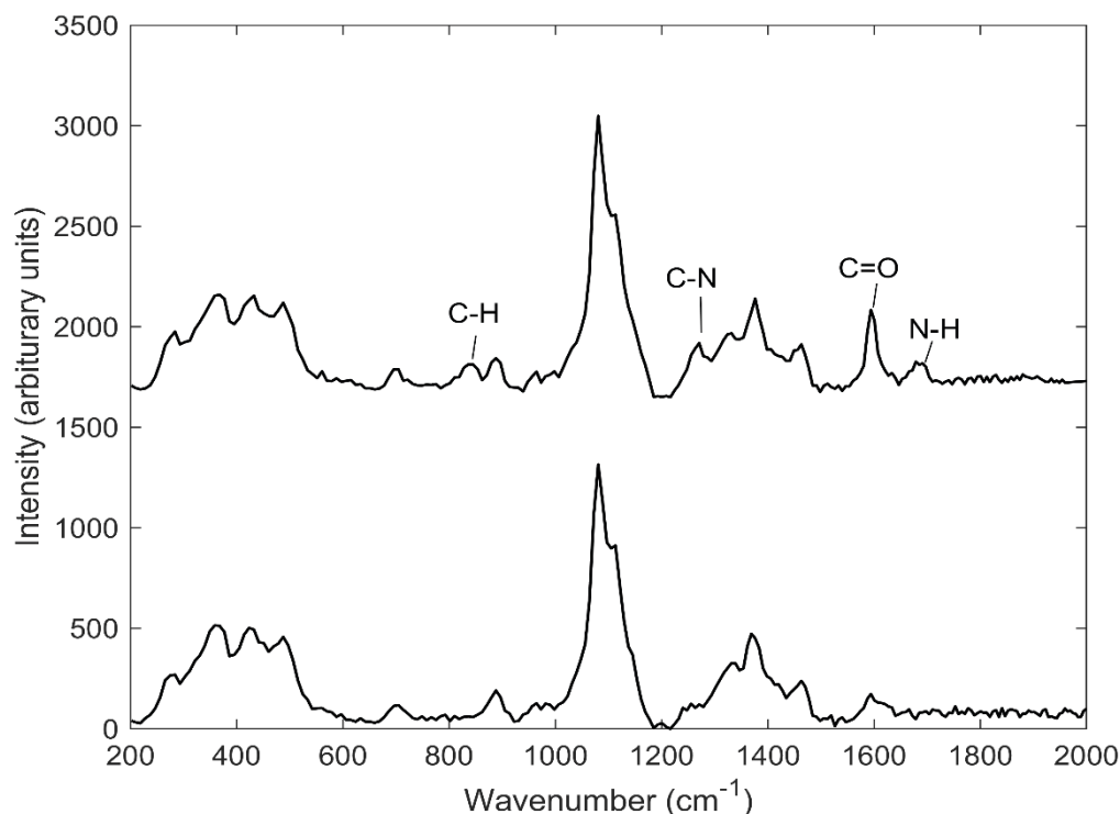
Figure 5. Raman stacked spectra of blank paper (bottom) and procaine (top) impregnated into paper at 25 mg/mL concentration measured in the wavenumber region 200 -2000 \text{cm}^{-1} . Only functional groups attributed to the drugs are labelled.
