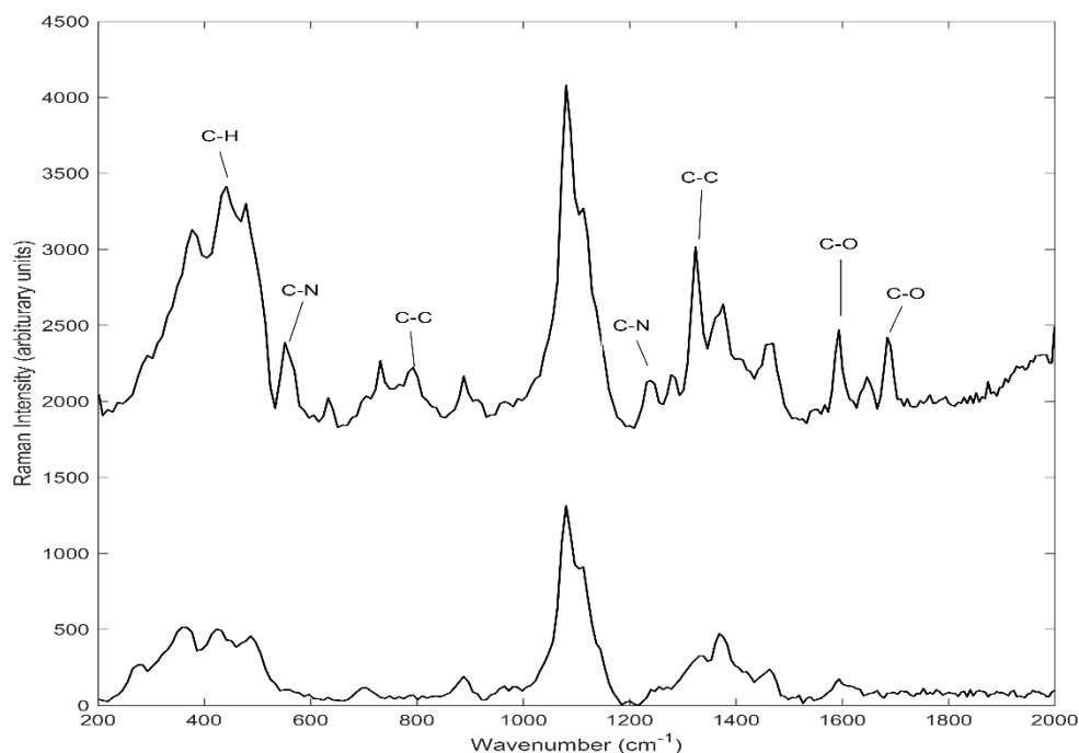
Figure 4. Raman stacked spectra of blank paper (bottom) and caffeine (top) impregnated into paper at 25 mg/mL concentration measured in the wavenumber region 200 -2000 \text{cm}^{-1} . Only functional groups attributed to caffeine were labelled.
