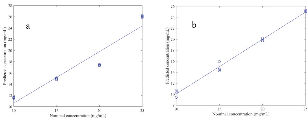
Figure 6- PLSR calibration models of the Raman spectra of (a) caffeine and (b) procaine HCl impregnated into paper.
