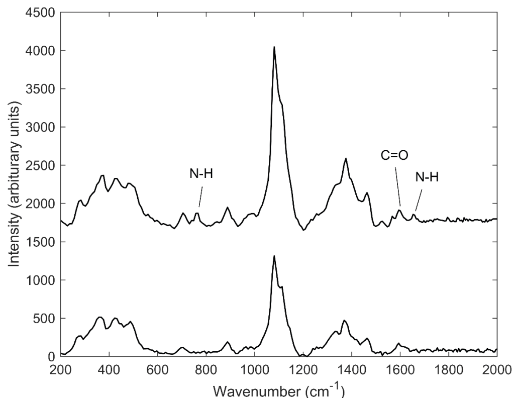
Figure 3. Raman spectra of blank paper (bottom) and AKB-48 (top) impregnated into paper at 25 mg/mL concentration measured in the wavenumber region 200-2000 \text{cm}^{-1} . Only functional groups attributed to the AKB-48 were labelled.
