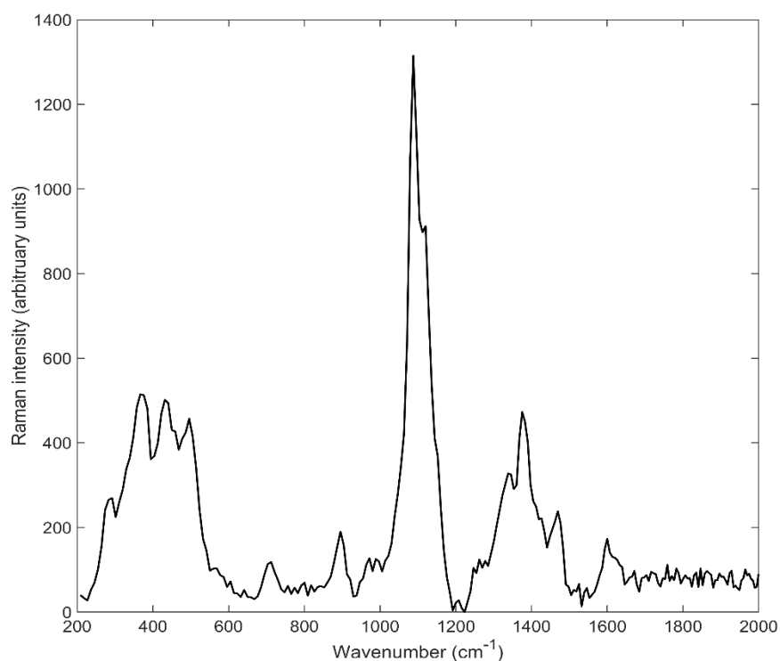
Figure 1. Raman spectrum of blank paper 80 g/m 2 measured using the Rigaku handheld FT-Raman spectrometer.
