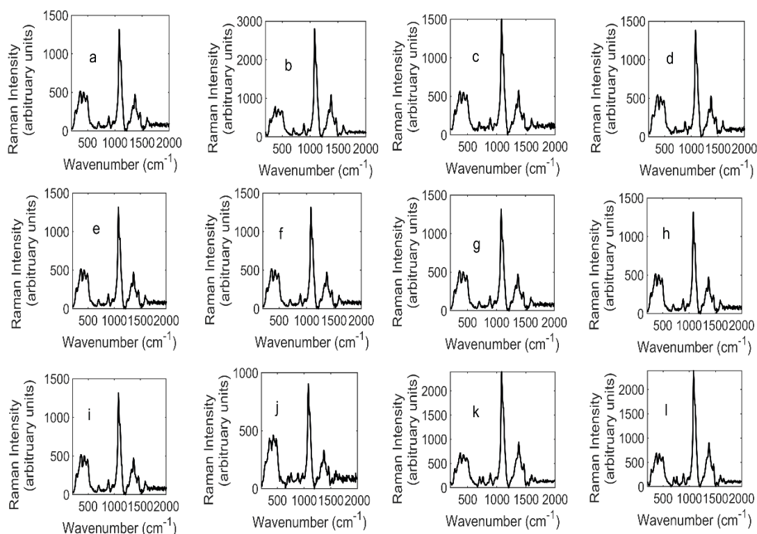
Figure 2. Raw Raman spectra of (a) 5F-PB-22 impregnated into paper at 10 \text{mg/mL} (b) 15 \text{mg/mL} (c) 20 \text{mg/mL} (d) 25 \text{mg/mL} , AB-FUBINACA 22 impregnated into paper at (e) 10 \text{mg/mL} (f) 15 \text{mg/mL} (g) 20 \text{mg/mL} (h) 25 \text{mg/mL} and AKB-48 22 impregnated into paper at (i) 10 \text{mg/mL} (j) 15 \text{mg/mL} (k) 20 \text{mg/mL} (l) 25 \text{mg/mL} measured by the handheld Rigaku FT-Raman spectrometer.
