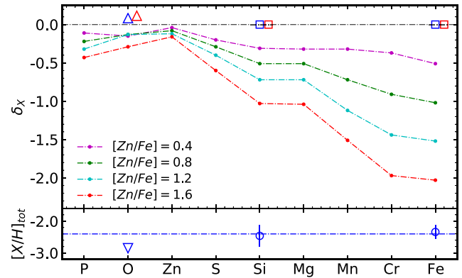
Figure 5. Dust depletion pattern and metallicity for the measured column densities of the features found in absorption in the afterglow of GRB 160410A. Squares (top panel) and circles (bottom panel) denote the Si and Fe lines meanwhile triangles refer to the limits we derive for the saturated O line. With a small offset for visualization purposes. The red squares denote the depletion \delta_x values obtained for the common velocity component to all the elements observed, blue squares are the depletion considering the total column density measured. For comparison, we plot with a dash-dotted line in different colours the dust depletion sequence obtained from the fitting of QSO-DLA absorption systems in De Cia et al. (2016). Bottom panel: Corresponding metallicity for the observed ions considering all the velocity components. The mean metallicity is shown with a dashed-dotted line.
