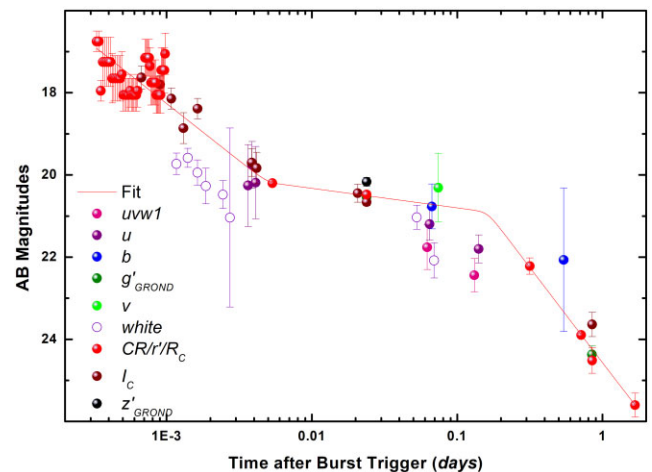
Figure 11. Light curve of the GRB 160410A afterglow. For reasons of clarity, upper limits are omitted. Early I_C data are from Trotter et al. (2016), the R_C data point at 0.31 d is from Wang et al. (2016), the rest from this work. Data are in the AB magnitude system and corrected for Galactic foreground extinction. The red line shows the modelled light curve for the CR/r'/R_C -band. A clear steep-shallow-steep transition is visible.
