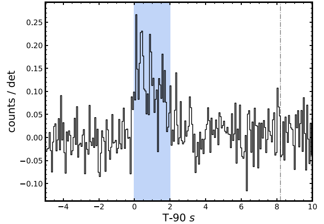
Figure A1. BAT mask-weighted light curve in the 15 to 350 keV range of GRB 160410A with 64 ms binning. The blue area marks a multipulsed structure during the first two seconds. The dash-dotted line marks the end of the T_{90} duration from Sakamoto et al. (2016) in the same energy band.
