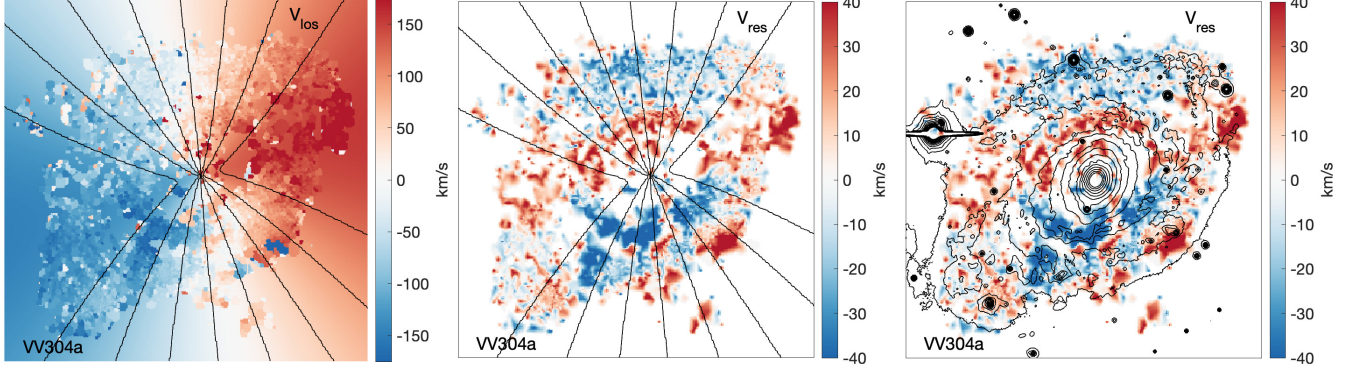
FIG. 3.— Left panel: Observed line-of-sight velocity field, V_{\text{los}} , of VV304a, derived from its H_\alpha emission. The smooth coloured background shows the modeled axisymmetric velocity field in regions without observable H_\alpha . The black lines show iso-velocity contours of this axisymmetric field. Middle panel: Residual velocity field, V_{\text{res}} , obtained from the difference between the observed and modeled V_{\text{los}} field. The transitions from positive to negative velocities along a given iso-velocity line are consistent with a corrugation pattern. These velocity fluctuations could indicate a significant displacement of the disc’s \langle Z \rangle with respect to its overall mid-plane. Right panel: Residual velocity field including isophotal contours obtained from r' -band optical image (Gemini/GMOS).
