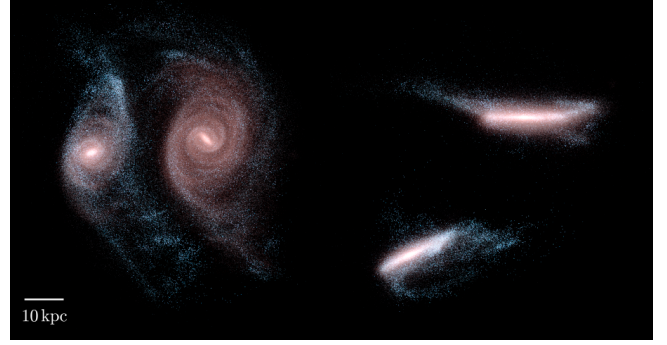
FIG. 7.— The moment of closest approach between the simulated Auriga galaxy, Au25, and its massive companion. The images were created as in Fig. 6. The face-on (left) and edge-on (right) views are oriented with respect to the Au25 disc. The disc shows a strong bar and a grand design spiral structure.
