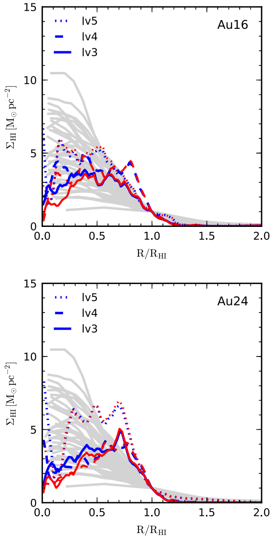
Figure 14. Resolution study for the H I surface density profiles for haloes Au 16 and Au 24. The blue and red lines indicate the profiles obtained using the prescription from L08 or GK11 for removing molecular gas, respectively. The line style indicates the resolution level, as given in the legend. Light grey lines display the H I radial profiles of the Bluedisk survey (Wang et al. 2014).
