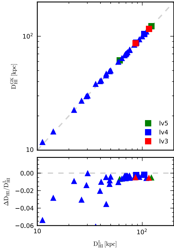
Figure 9. H I diameter mass obtained by using the L08 and the GK11 prescription to account for the molecular gas for the 30 Auriga haloes. Top panel: comparison of the H I diameters obtained in the two cases. Bottom panel: fractional variation with respect to the L08 H I diameter as a function of the L08 H I diameter. Dashed lines in both panels show the 1:1 correspondence.
