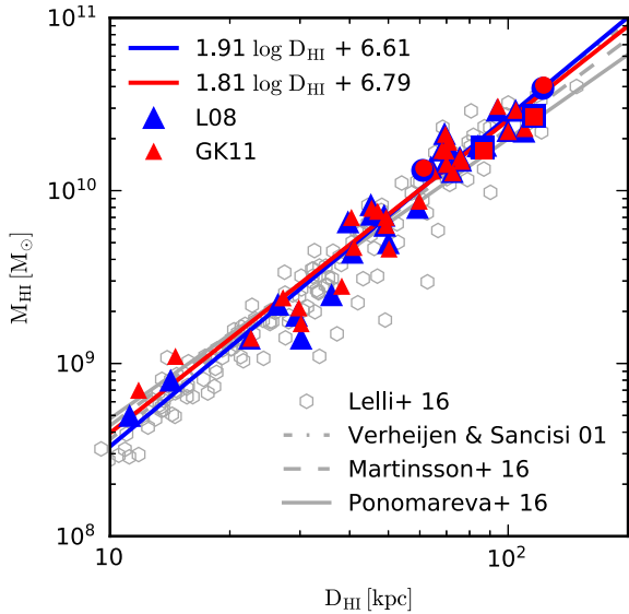
Figure 11. The H I mass diameter relation for the Auriga galaxies. Blue symbols show the results obtained with the empirical relation from L08 to account for molecular gas, while red symbols show the outcome of the prescription described in GK11 with lines of the same colours indicating the best-fitting relation inferred from the two samples. Grey lines and empty symbols, instead, compare the Auriga findings to observations of nearby galaxy as shown in the legend. Triangles present the results obtained at the standard (level 4) resolution, while circles and squares show haloes Au 16 and Au 24 at resolution levels 5 and 3, respectively, a factor of 8 coarser or finer in mass resolution (see also Section 4.7).
