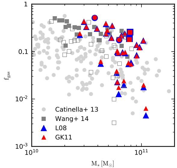
Figure 12. H I gas fraction as a function of the stellar mass for the Auriga sample. Stellar masses are computed within 10 per cent of the virial radius of each object, while H I masses are those listed in Table 1. Results obtained through the empirical relation in L08 to account for molecular gas are shown with red symbols, while those obtained by applying the GK11 prescription are represented by blue symbols. Triangles give the results obtained at the standard (level 4) resolution, while circles and squares show haloes Au 16 and Au 24 at resolution levels 5 and 3, respectively, a factor of 8 coarser or finer in mass resolution (see also Section 4.7). Grey symbols indicate observational findings from the GALEX Arecibo SDSS Survey (GASS; Catinella et al. 2013) and the Bluedisk (Wang et al. 2014) surveys, as indicated in the legend. For the combined data sets, only 195 out of 300 galaxies which were significantly detected in H I are shown.
