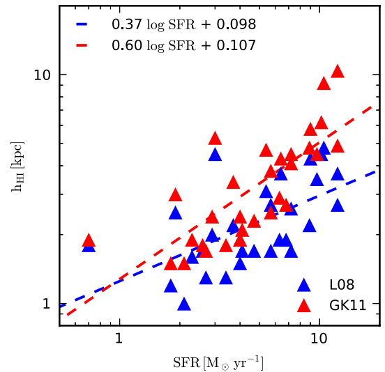
Figure 8. H I vertical thickness (defined as the height containing 75 per cent of the H I mass) as a function of the SFR within the galaxy B -band optical radii for the 30 Auriga haloes derived with the L08 (blue symbols) and GK11 (red symbols) prescriptions for the treatment of molecular hydrogen. Dashed lines represent the best-fitting relations in the two cases, with parameters indicated in the legend.
