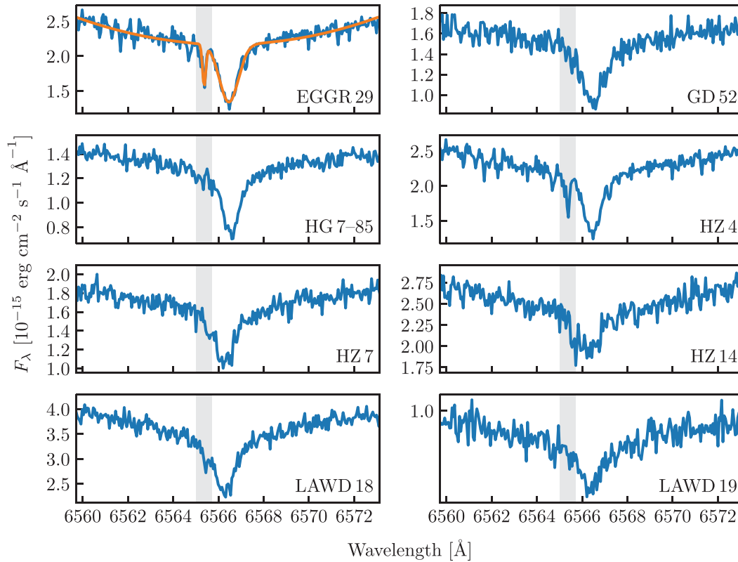
Figure 1. Close-up on the H\alpha NLTE core of sample ESPRESSO spectra for the eight Hyades WDs. As an example, for the top left-hand spectrum (EGGR 29), the best-fitting model is overplotted in orange. The photospheric H\alpha is modeled with a quadratic polynomial and the NLTE core with a Gaussian. In some spectra a second narrow absorption line, whose position is highlighted by the grey band, is visible on the blue side of the core (see e.g. HZ 4 and EGGR 29), resulting from the imperfect subtraction of the H\alpha sky emission line. We fitted this residual with a second Gaussian. Without it, the measured \Delta V would have been systematically smaller.
