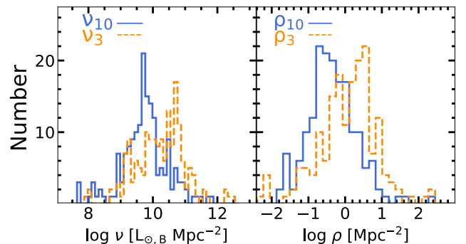
Figure A1. Histogram of the luminosity surface densities ( \nu_{10} and \nu_3 ) and surface densities ( \rho_{10} and \rho_3 ) for our sample of 173 LeMMINGS galaxies.
