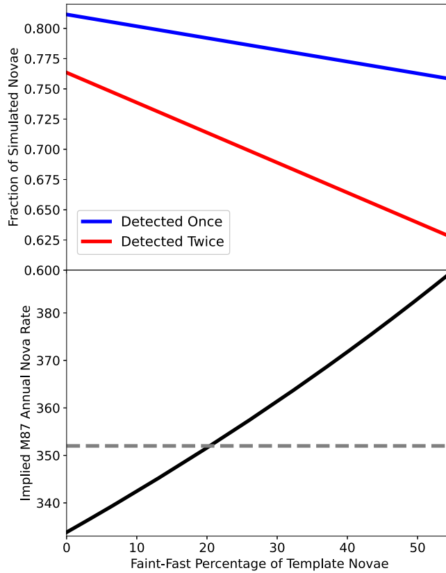
Figure 3. Top: the fraction of simulated novae detected once (blue) and twice (red) in F606W as a function of the percentage of template novae that are faint, fast ( t_2 < 10 days and peak M(F606W) < -7 ). Bottom: the annual nova rate for the entirety of M87 implied by the recovery fraction, following the procedure of Section 4.5. Also shown (horizontal line) is the annual nova rate adopted in Section 4.5.
