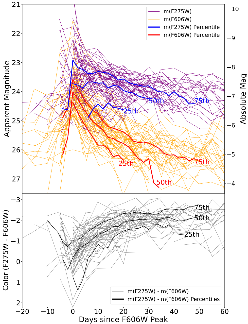
Figure 5. Top: F275W and F606W light curves (purple and orange, respectively) of 77 novae with brightness peaks in M87. Over-plotted are the 25th, 50th, and 75th percentiles (in order of brightness) of all of these F275W (in blue) and F606W (in red) light curves. Note that the computation of a percentile at a given time takes into account upper limit magnitude data points in individual nova light curves. To avoid clutter in this plot, those individual limit data points are not shown, but they can be seen in Table 3 and as arrows in Figure 15. The higher luminosities and slower rates of decline of novae in the NUV are apparent. Bottom: the F275W–F606W color curves of the M87 novae, as well as the 25th, 50th, and 75th percentiles of the color curves. Novae near maximum light exhibit m(\text{F275W})-m(\text{F606W}) \sim 0 \pm 1 , then become increasingly blue during the ensuing \sim 30 days. After \sim 30 days they remain at m(\text{F275W})-m(\text{F606W}) \sim -2 \pm 0.5 .
