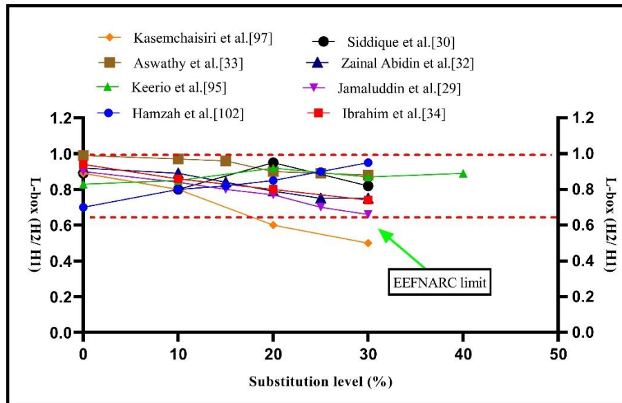
Fig 5. L-box values' variation in SCC using varying CBA replacement ratios
