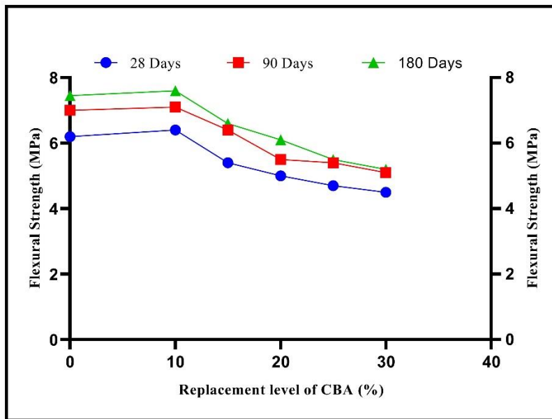
Fig 7. Flexural strength of samples with various replacement ratios in SCC at different curing ages [37]
