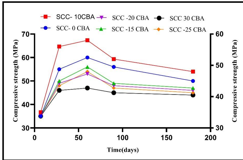
Fig 6. The samples' compressive strength with varying replacement percentages in SCC [108]
