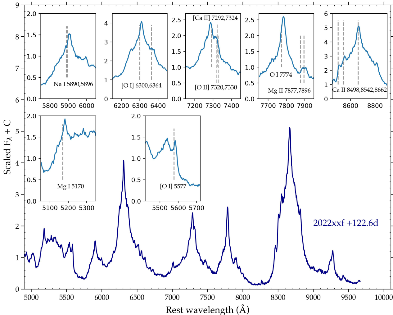
Fig. 5. Nebular spectrum of SN 2022xxf at +122.6 days. Insets show close-ups of the emission lines, with dashed vertical lines indicating the rest wavelengths of the emitting species.
