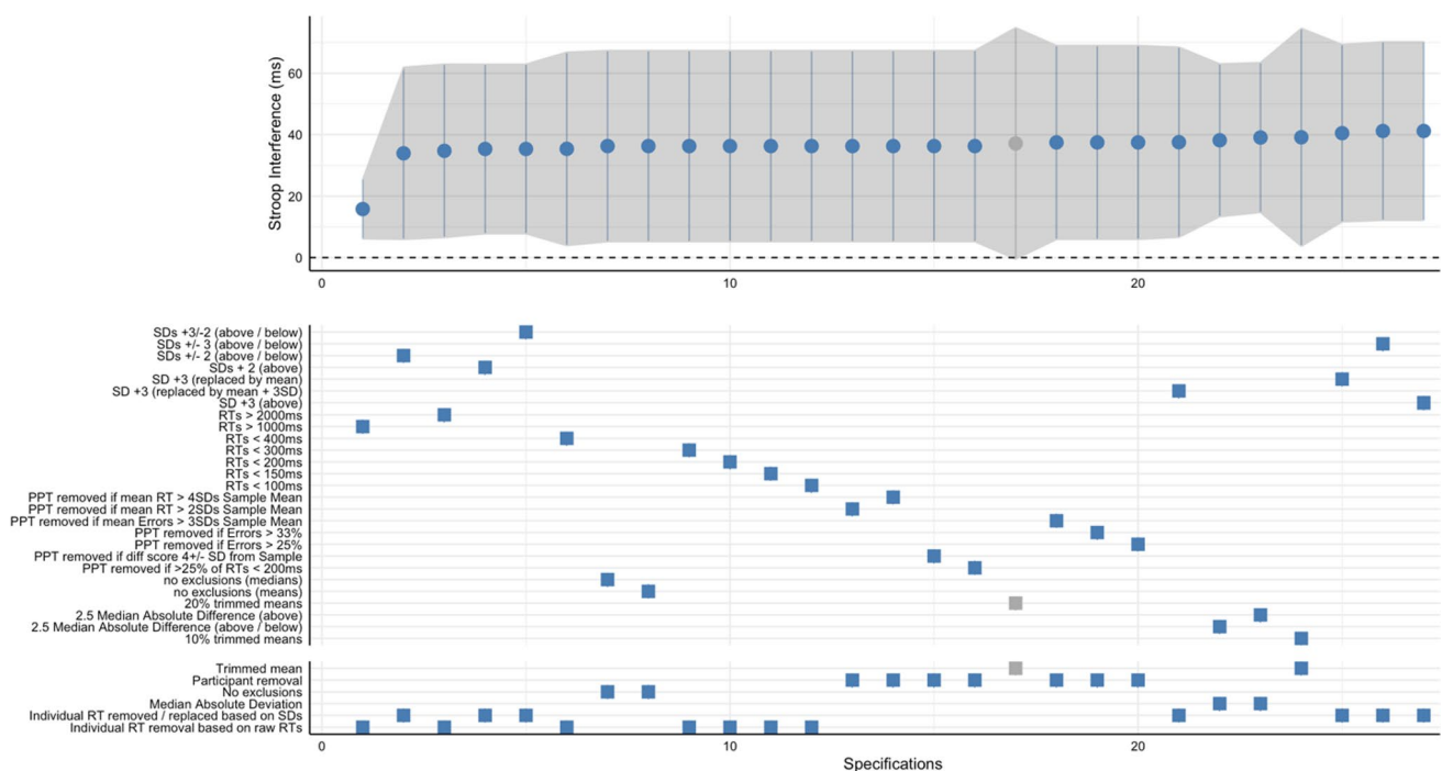
Fig. 1 Specification curve for the analysis decisions of the Stroop data published in Spanakis et al. (2019). The outcome is the Stroop interference effect (difference in RTs for alcohol – emotionally neutral words)
