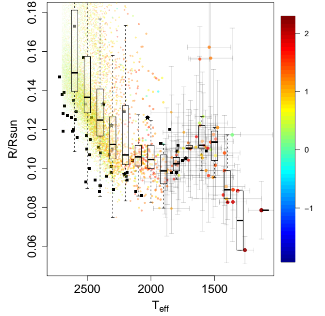
Fig. 17. Radii of candidate UCDs in the Gaia golden sample. The colour code indicates the logarithm of the VOSA fit \chi^2 values, squares represent the data points in Table 1 of Dieterich et al. (2014), and black asterisks denote unresolved binaries therein. The box plots are calculated within bins of 100 K.
