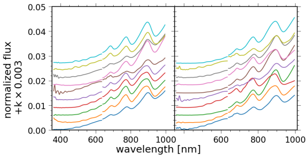
Fig. 26. BP and RP spectra of the 20 randomly chosen (amongst 254) carbon stars (this work) with T_{\text{effGSP-Phot}} > 6000 K. The ordinate axis provides the flux normalised to the total flux, and shifted by k \times 0.003 (where k is an integer that varies from 0 to 9 from the bottom to the top spectrum).
