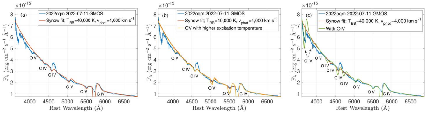
Figure 5. SYNOW fits to the first high-spectral resolution spectrum (GMOS; t = 0.7 day). All fits assume a 40,000 K continuum and an expansion velocity of 4000 \text{km s}^{-1} . (a) C IV and O V using the default parameters of SYNOW. (b) The same as (a) but with a higher specific excitation temperature for O V. (c) The same as (a), but also including O IV.
