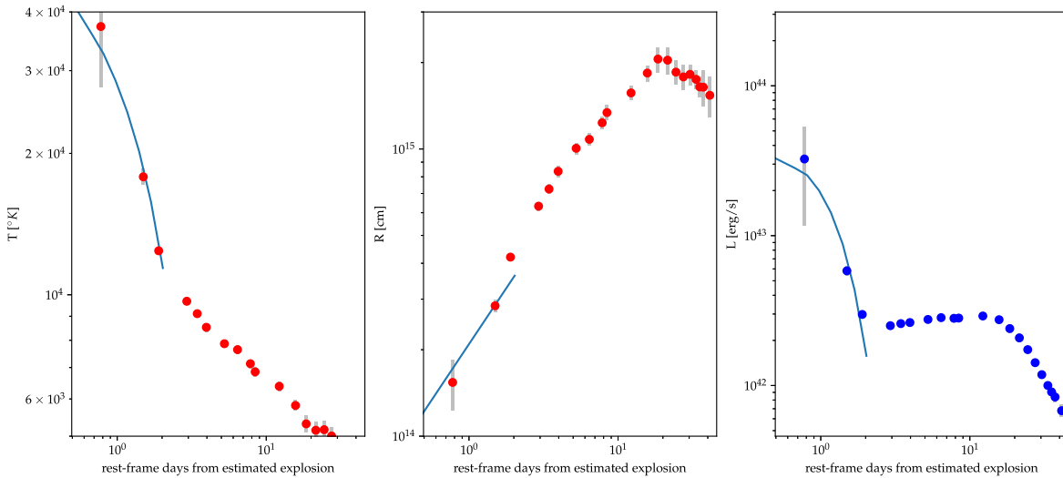
Figure A5. The blackbody evolution of the best-fitting shock-cooling Piro et al. (2021) model with the blackbody evolution of SN 2022oqm. The models are plotted up to t = t_{ph} , when the envelope becomes fully transparent.
