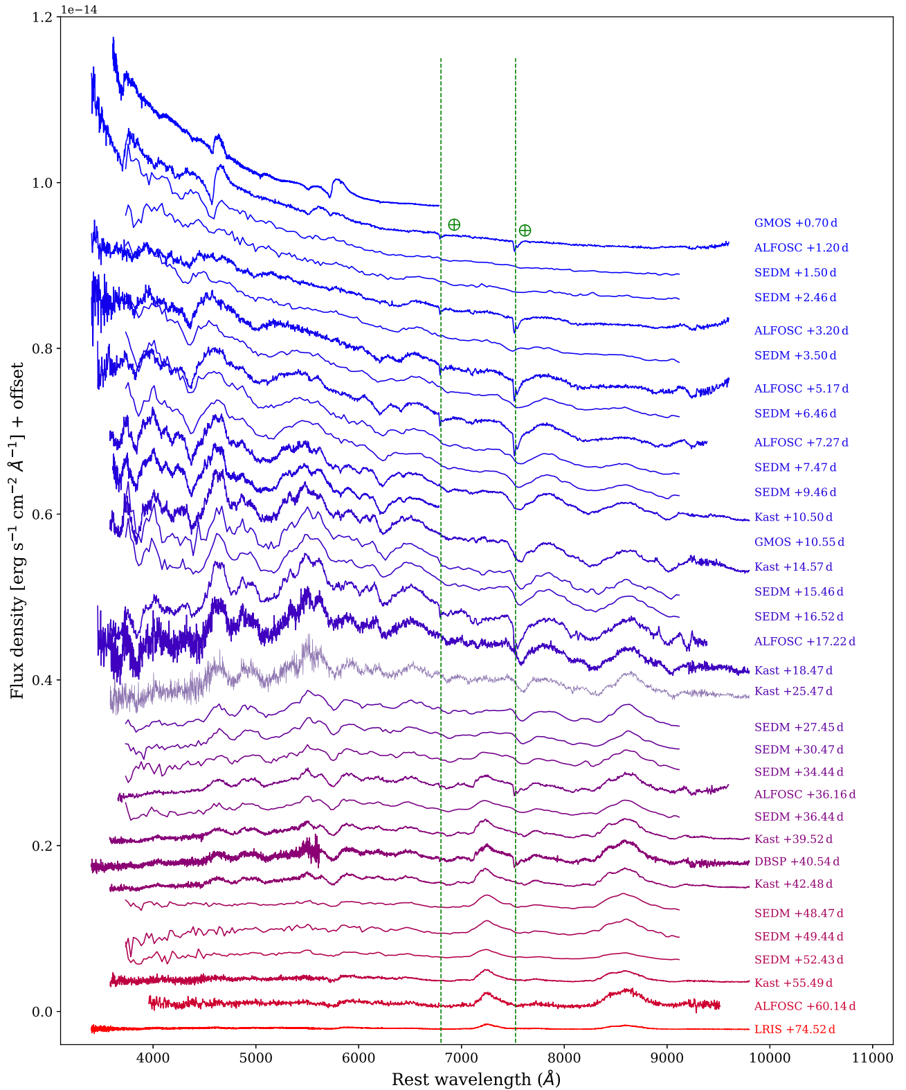
Figure 2. Spectral evolution of SN 2022oqm. The phases are reported relative to the estimated explosion time of JD = 2,459,771.217 . The locations of telluric features are marked with vertical green-dashed lines.
