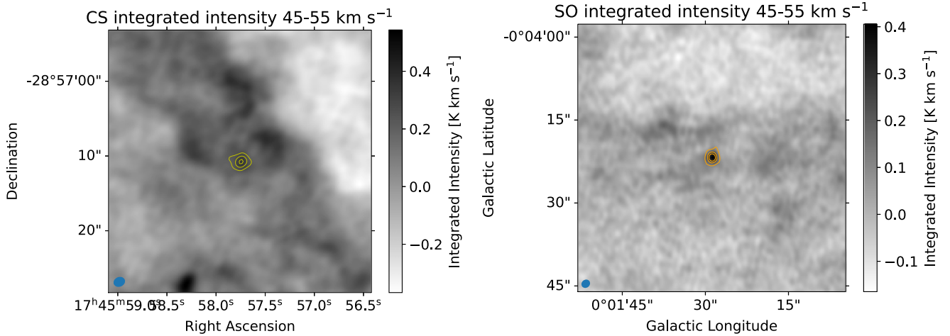
Figure 10. In both images, the gray scale shows the integrated intensity over the range 45–55 km s −1 . The left image shows CS 2–1, and the right shows SO 2(3)–1 (2). The contours show the MUBLO integrated over the full velocity range but with contaminated velocities masked out; the contours are at 20, 40, and 60 K km s −1 (CS; left) and 20, 60, and 100 K km s −1 (SO; right). These images provide context on where the compact source resides. The MUBLO is not detected in CS over the narrow velocity range because the “diffuse” molecular gas at that velocity dominates over the compact source, while the MUBLO is still well detected in SO over the same velocity range, presumably because the SO 1(2) level (the lower state of the SO 2(3)–1(2) transition) is un- or underpopulated in the diffuse cloud.
