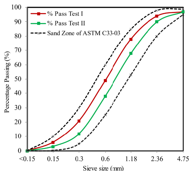
Fig. 1. Sand sieve analysis result
