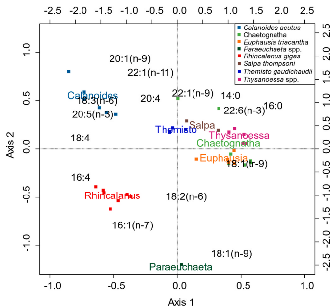
Fig. 7. Fatty acid composition (mol%) of the zooplankton taxa from station P3 (P3B + P3C) in the Scotia Sea. Redundancy analysis distance triplot of the proportional abundance of fatty acids in each sampled zooplankton taxa and 16 fatty acids. The primary and secondary sets of axes relate to the individual zooplankton samples and fatty acid loadings, respectively. Each single point refers to an individual taxon replicate.
