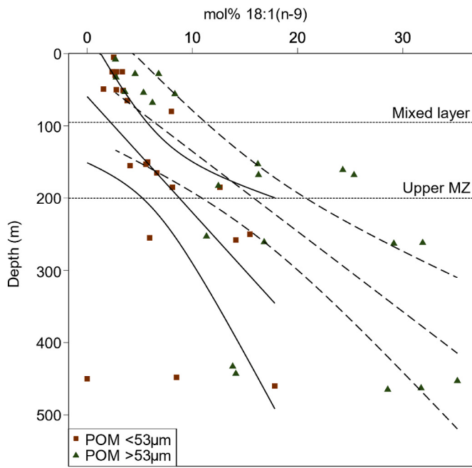
Fig. 4. Relationships between depth and the relative abundance of the biomarker 18:1(n-9) (mol%) fatty acid in the <53 \mu\text{m} (filled squares) and >53 \mu\text{m} (filled triangles) size-fractions of particulate organic matter (POM) sampled at station P3 (P3A + P3B + P3C) in the Scotia Sea. This fatty acid is biosynthesized by animals (Dalsgaard et al., 2003), but not phytoplankton, and is therefore representative of zooplankton-sourced materials to the particle pool and more reworked POM. The regression lines indicate statistically significant ( p < 0.05 ) linear relationships. POM <53 \mu\text{m} (solid line): y = 16.06x (\pm 5.61) + 59.44 (\pm 43.92) ( R^2 = 0.29 ); POM >53 \mu\text{m} (dashed line): y = 11.08x (\pm 2.28) + 24.41 (\pm 43.19) ( R^2 = 0.54 ). Standard errors are illustrated either side of the regression line and given in brackets next to the equation coefficients. Horizontal dotted lines indicate the boundaries of the mixed layer depth (0–95 m) and the upper mesopelagic zone (MZ) (96–200 m) (Giering et al., 2023).
