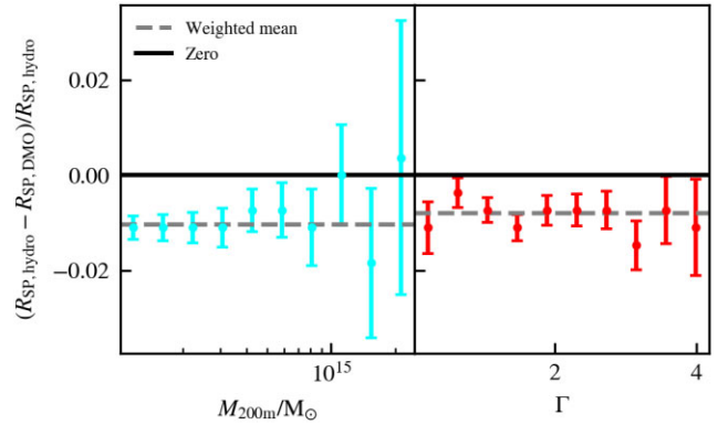
Figure 5. Comparison of the splashback radius extracted from the L1_m9 and L1_m9_DMO simulations when stacking the dark matter density profiles into bins of mass (left panel) and accretion rate (right panel). The error bars show the uncertainty by propagating the bootstrap error of the splashback radius from both the DMO and hydro simulations.
