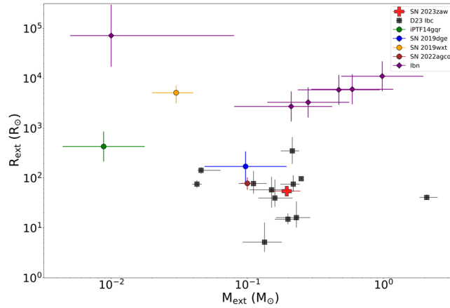
Figure I1. The envelope properties of SN 2023zaw (red cross) compared with double-peaked Type Ibc SNe (black squares) from Das et al. (2023b), USSN candidates (circles)—iPTF14gqr, SN 2019dge, SN 2019wxt, SN 2022agco (De et al. 2018b; Yao et al. 2020; Agudo et al. 2023; Shivkumar et al. 2023; Yan et al. 2023), and Type Ibn SNe (purple diamonds)—SN 2006jc, SN 2019wep, SN 2019up, SN 2012jpk, SN 2019deh, LSQ13ddu (Anupama et al. 2009; Clark et al. 2020; Pellegrino et al. 2022).
