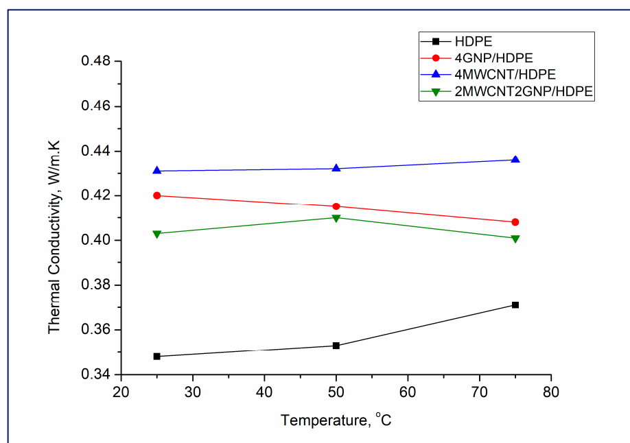
Figure 5. Thermal conductivity of the composite materials as a function of the testing temperatures.
