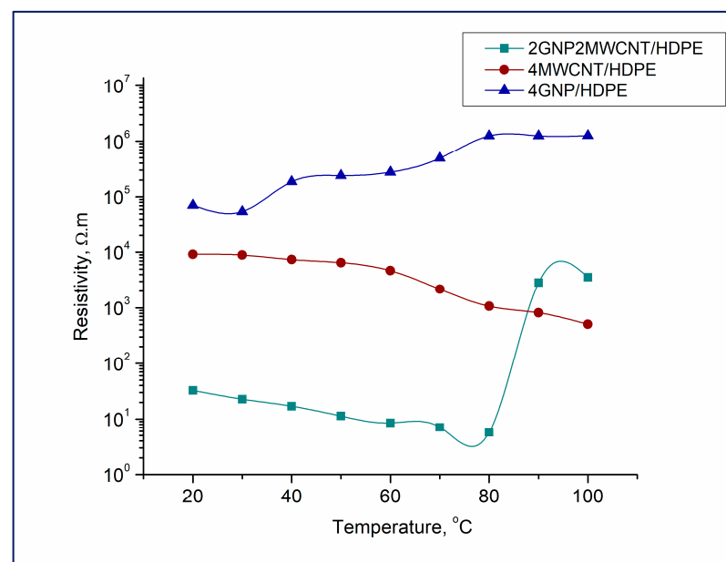
Figure 6. Resistivity measurements of the nanocomposite structures in the temperature range of 20–100 °C.
