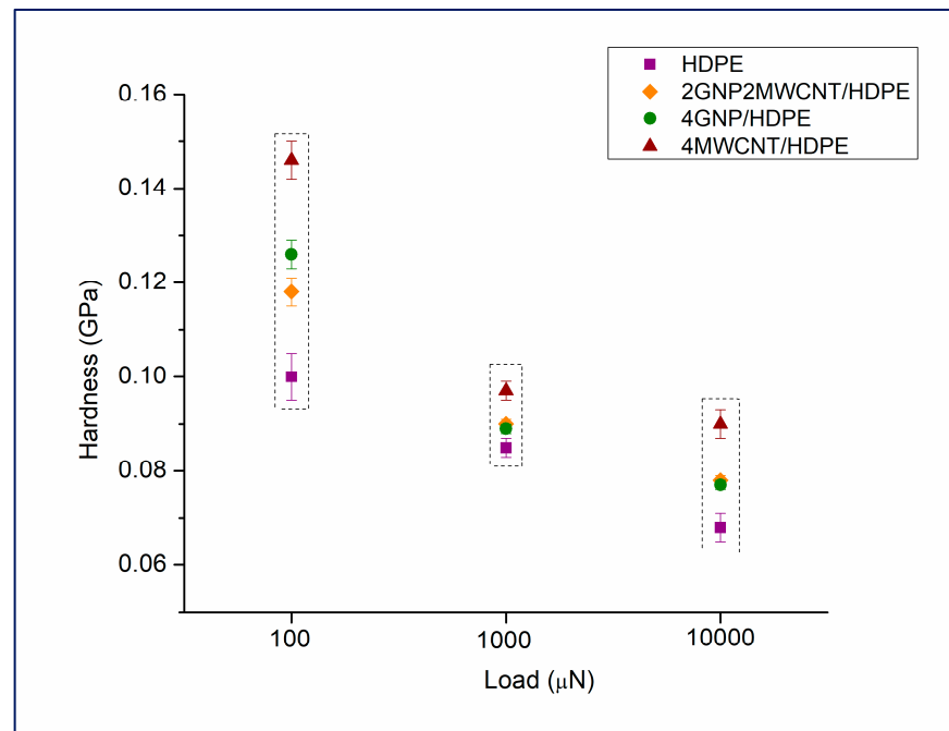
Figure 1. Nanohardness of the nanocomposite samples, including pure HDPE as a reference, measured at three different peak loads—100 \mu\text{N} , 1000 \mu\text{N} , and 10,000 \mu\text{N} .
