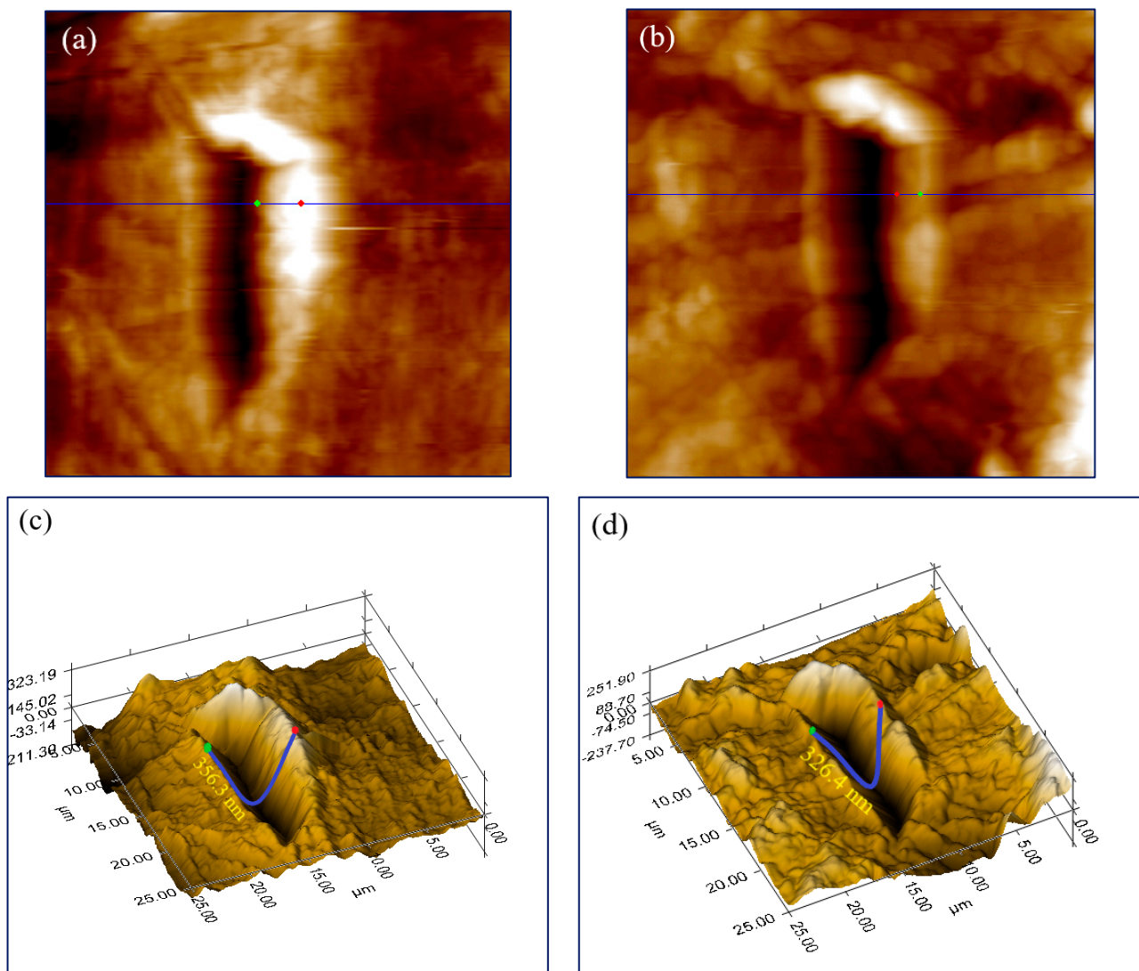
Figure 4. In-situ SPM topography forward and 3D plot imaging of nanoscratch grooves over the surface of pure HDPE (pictures (a,c)) and over a hybrid composition of 2wt%GNP2wt%MWCNT/HDPE (pictures (b,d)).
