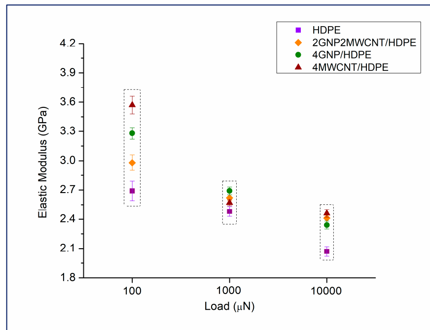
Figure 2. Reduced modulus of elasticity of the nanocomposite samples, including pure HDPE as a reference, measured at three different peak loads—100 \mu\text{N} , 1000 \mu\text{N} , and 10,000 \mu\text{N} .
