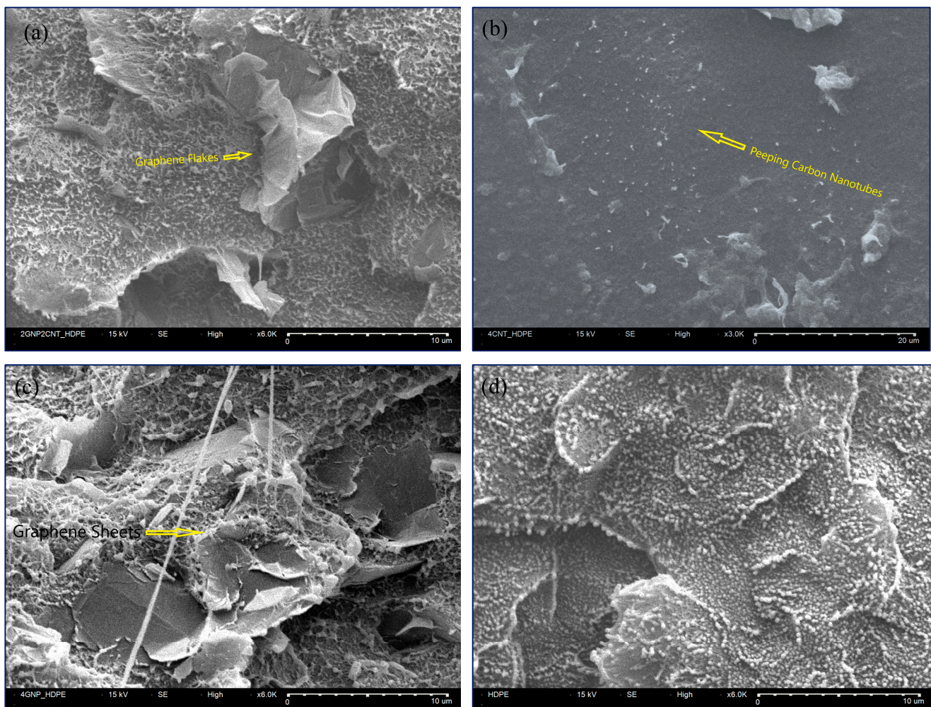
Figure 7. SEM micrographs of the following specimens: 2wt%GNP2wt%MWCNT/HDPE (a), 4wt%MWCNT/HDPE (b), 4wt%GNP/HDPE (c), and the pure HDPE as a reference (d).
