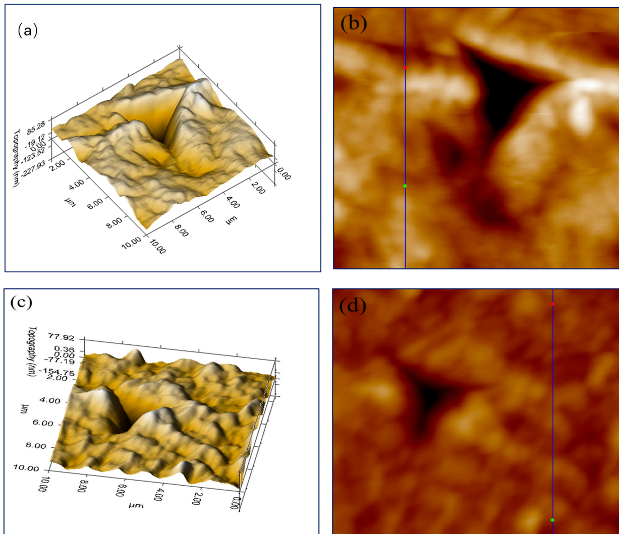
Figure 3. 3D plots of indentation imprints on the surface of neat HDPE (a) and 4wt%MWCNT/HDPE nanocomposite sample (c) as well as topography forward images of the same indentation surface areas (b) and (d) made by in-situ SPM imaging, including estimation of average surface roughness.
