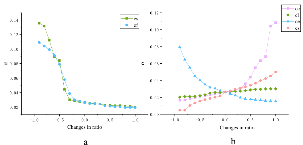
Figure 10. Sensitivity analysis on the empty-laden ratio.
