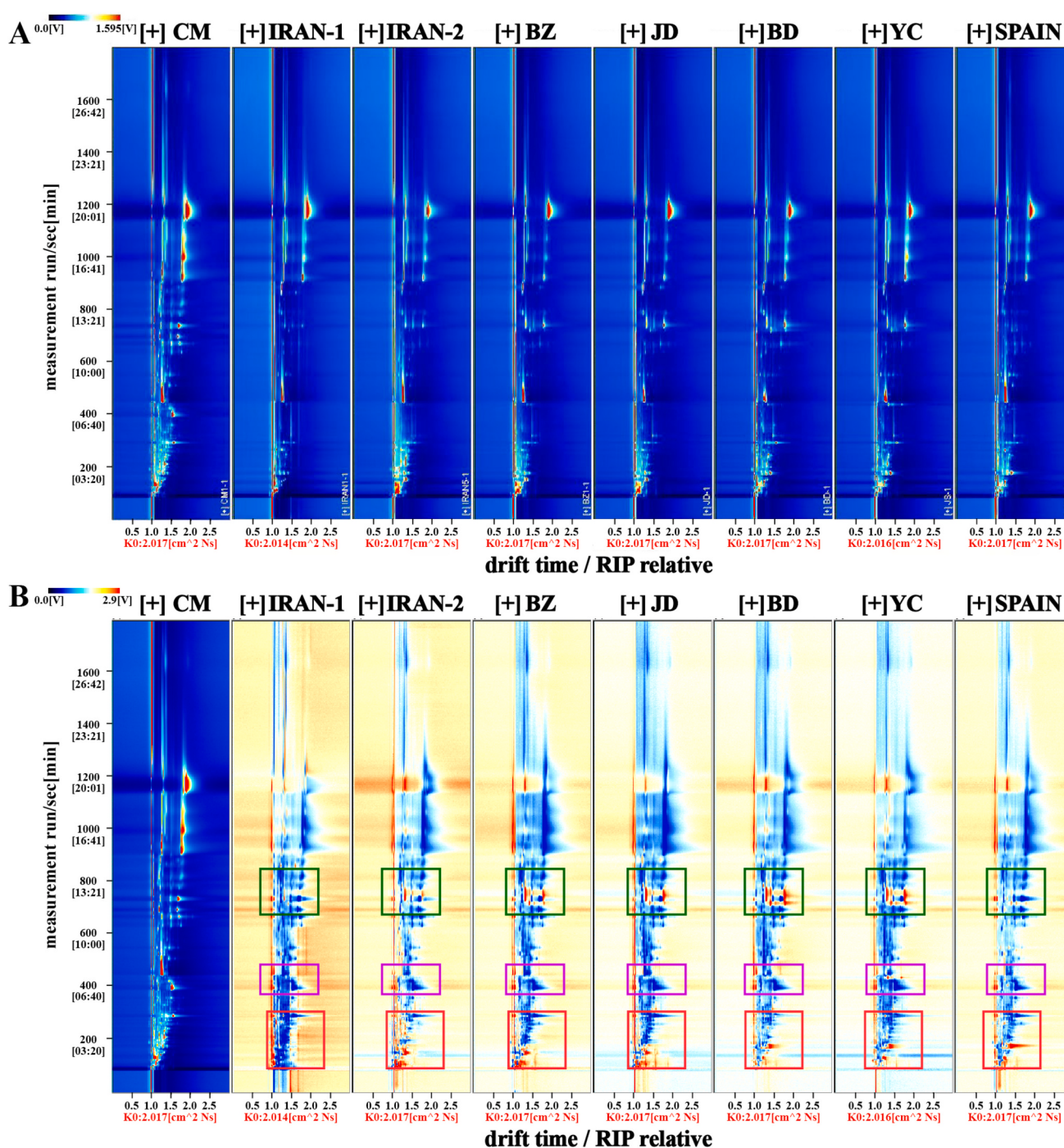
Fig. 2. (A) 2D Topographical map of saffron from different origins; (B) Differential spectra of saffron samples with saffron from Chongming as a reference.
