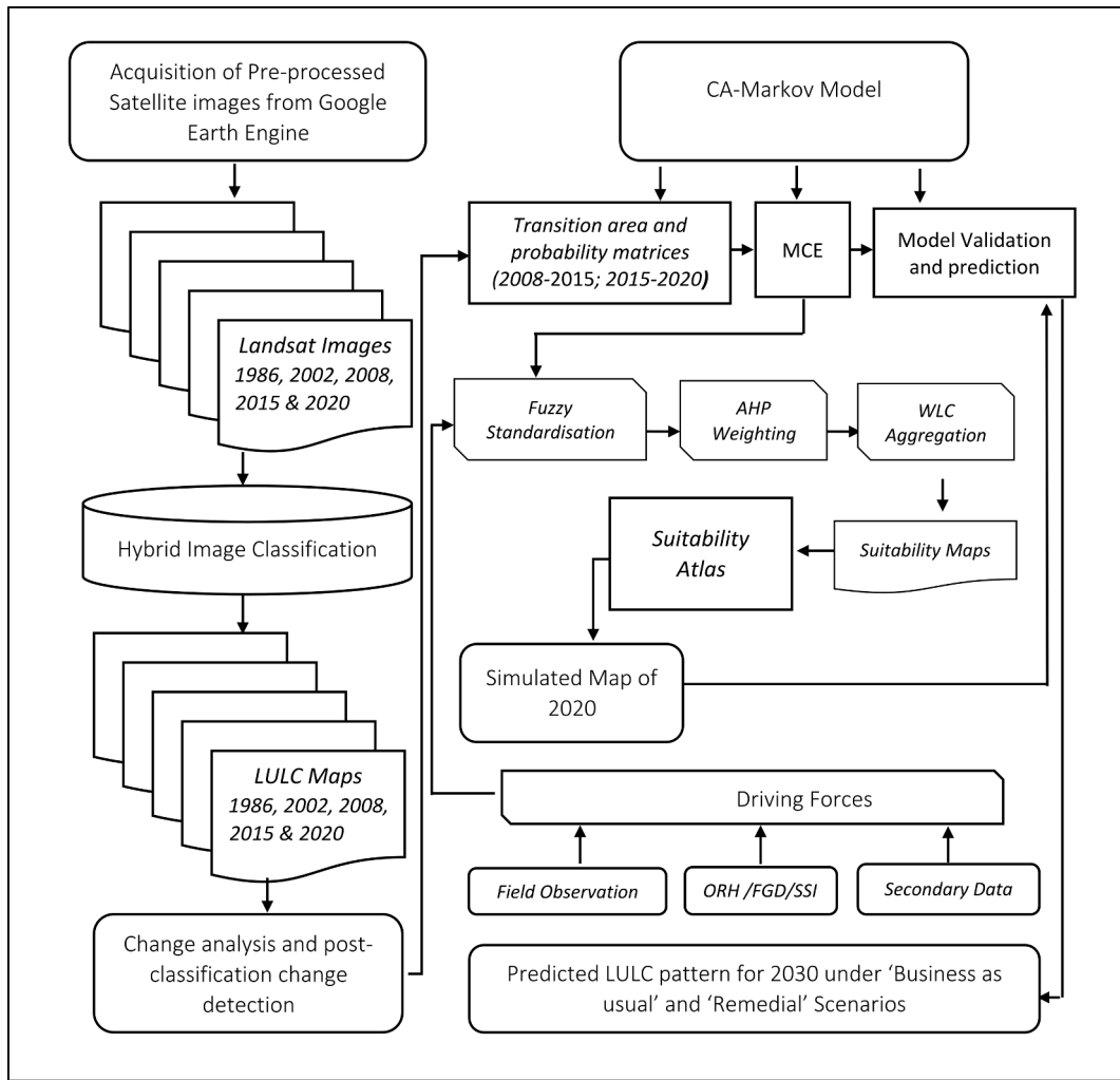
Fig. 1. Methodological Flowchart
