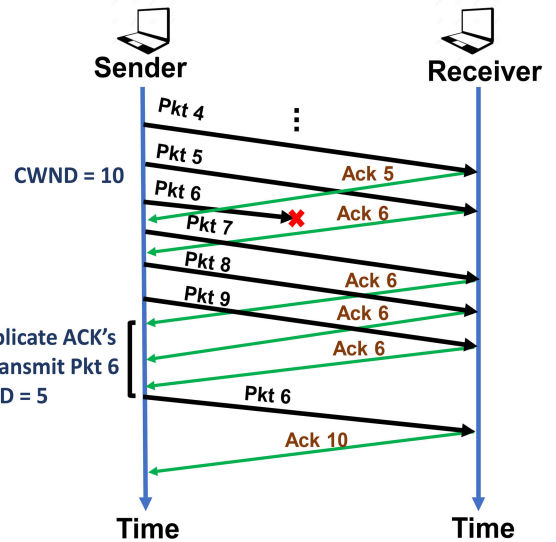
FIGURE 1. Pkt transmission, ACK receiving timeline showing 3 duplicate ACK's.
