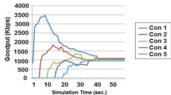
FIGURE 15. Intra-Algorithm fairness comparison.
