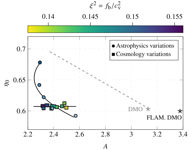
Figure 9. Best-fitting values of the two parameters, A and \eta_0 , used in the HM-CODE model to describe the effect of baryons on the matter power spectrum, obtained by fitting the model to the suppression of the power spectrum in the FLAMINGO simulations. The circles correspond to simulations that vary astrophysical parameters at fixed cosmology, while the squares correspond to simulations that vary cosmological parameters with fixed subgrid parameters. The lighter star labelled DMO marks the parameters in the absence of baryonic effects and the grey dashed line is a fit, \eta_0 = 0.98 - 0.12A , from Joudaki et al. (2018) to feedback variations from the OWLS suite (Schaye et al. 2010). The darker star marks the best-fitting parameters for the fiducial gravity-only FLAMINGO simulation.
