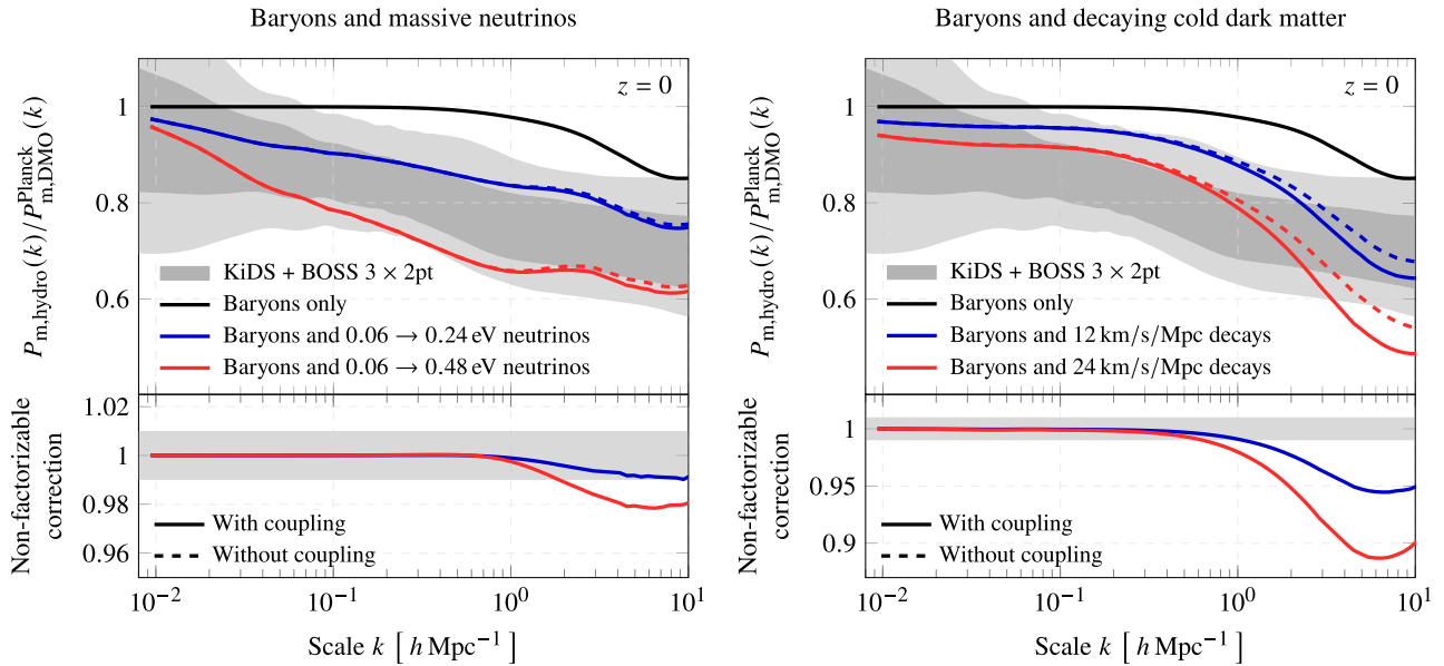
Figure 7. Matter power spectra relative to the spectrum for a Planck -based \Lambda CDM cosmology (Aghanim et al. 2020) without baryonic effects. The shaded contours in the top panel show the 68 per cent and 95 per cent ranges of \Lambda CDM spectra obtained from the 3 \times 2 pt KiDS + BOSS + 2dFLenS analysis (Heymans et al. 2021), which include the effects of baryonic feedback by marginalizing over a halo model-based feedback parameter (Mead et al. 2015; see Section 5). The left panel shows the effects of baryons alone and the effects of baryons combined with changing the neutrino mass from \sum m_\nu = 0.06 to 0.24 eV or 0.48 eV. The solid lines represent the simulation results, while the dashed lines show the results without accounting for the cosmology dependence of baryonic feedback. The right panel shows the same for decaying cold dark matter (DCDM) models with decay rates of \Gamma = 12 \text{ km s}^{-1} \text{ Mpc}^{-1} and 24 \text{ km s}^{-1} \text{ Mpc}^{-1} . The bottom panels show the non-factorizable corrections, i.e. the ratios of the solid and dashed curves in the top panels, with shaded bars representing a 1 per cent error.
