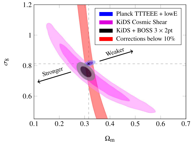
Figure 6. The cosmological parameters for which the baryonic suppression of matter clustering is similar to that in the best-fitting Planck model. This corresponds to the range where absolute errors to the matter power spectrum are \lesssim 1 per cent, or more precisely where relative non-factorizable corrections, \Delta F_b/(1 - F_b) , are below 10 per cent on scales 0.1 h \text{ Mpc}^{-1} \leq k \leq 10 h \text{ Mpc}^{-1} at z = 0 . The arrows indicate where baryonic feedback is at least 10 per cent stronger than in the Planck model (lower \sigma_8 and \Omega_m ) and weaker (vice versa). This is to be compared with the marginal posteriors from KiDS-1000, KiDS + BOSS + 2dFLenS, and Planck TTTEEE + lowE.
