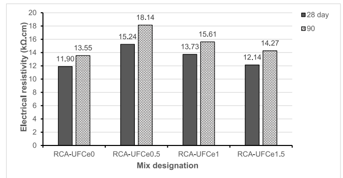
Fig. 14. RCA concrete mix electrical resistivity value with and without UFCe at 28 and 90 days.
