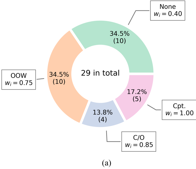
Fig. 3. FGCM example.
