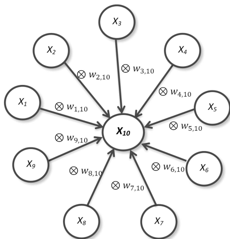
Fig. 4. Proposed FGCM.
