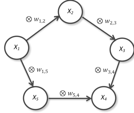
Fig. 3. FGCM example.
