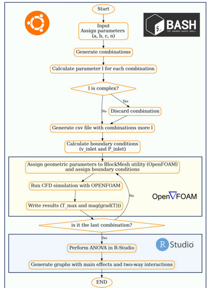
Fig. 5. Flowchart optimization algorithm.
