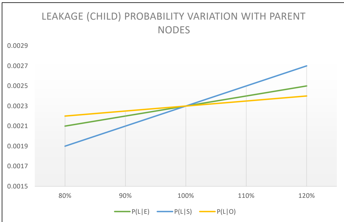
Figure 8. Leakage probability changes with parent nodes.
