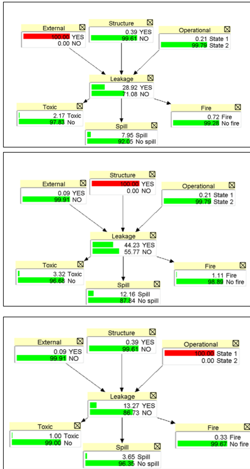
Figure 6. Leakage and consequence changes with parent nodes.
