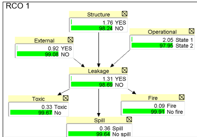
Figure 14. Bayesian network after applying RCO 1.
