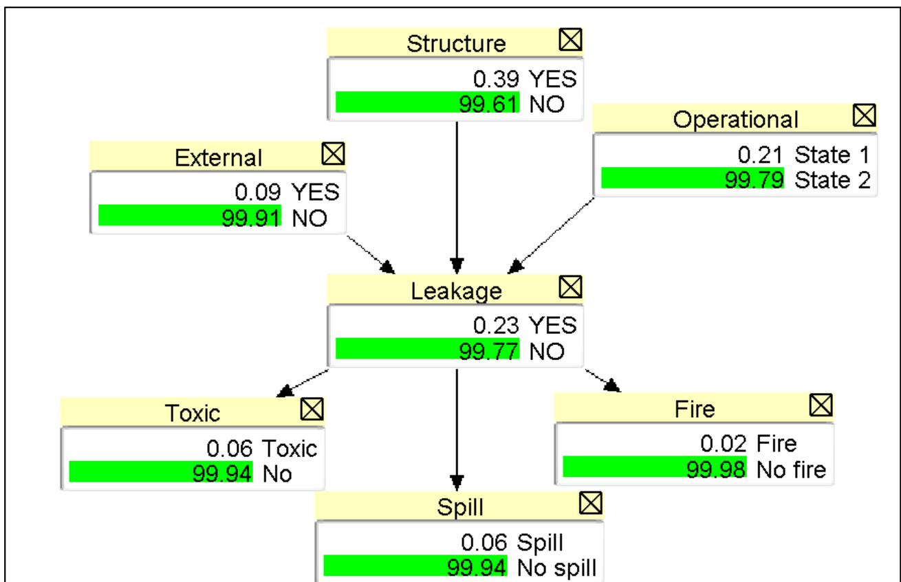
Figure 5. Ammonia leakage network.
