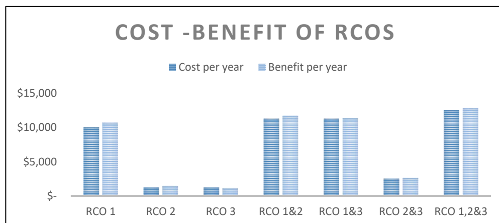
Figure 16. Cost-benefit of RCOs.
