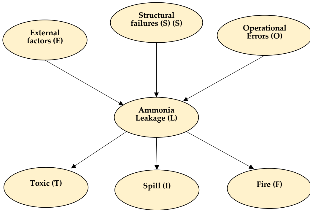
Figure 4. Proposed BN structure.
