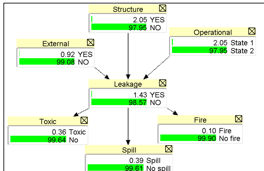
Figure 13. BN after five years of operation.
