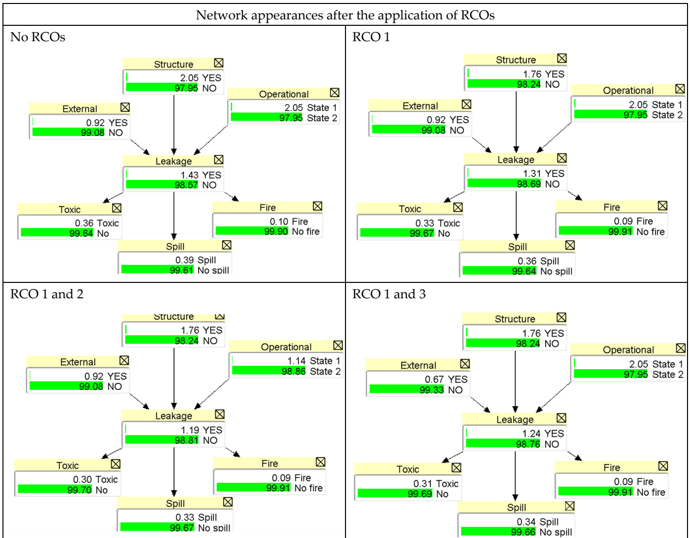
Figure 15. BN updates with combinations of RCOs.
