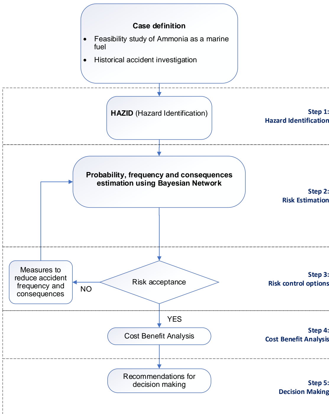
Figure 2. Research methodology.
