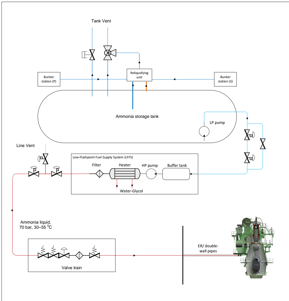
Figure 3. Proposed ammonia storage facility.
