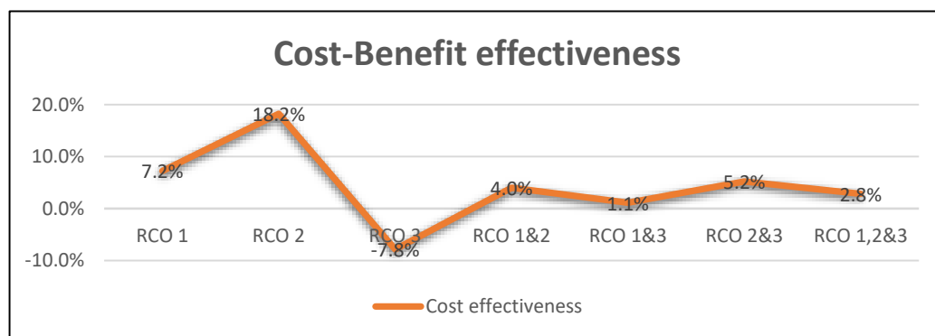
Figure 17. Cost–benefit effectiveness of RCOs.
