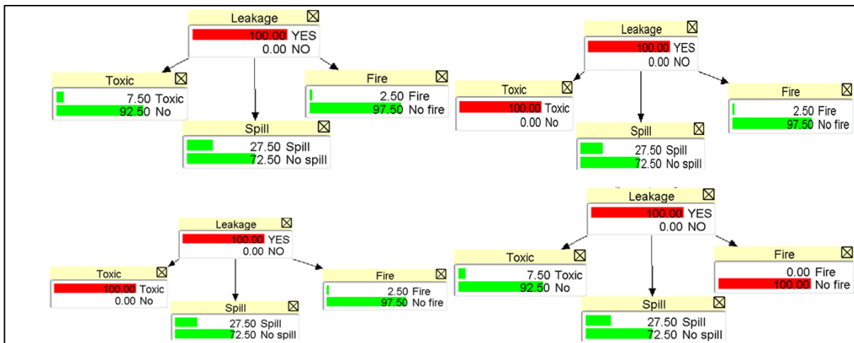
Figure 11. Divergent-type nodes with parent nodes' state evident.
