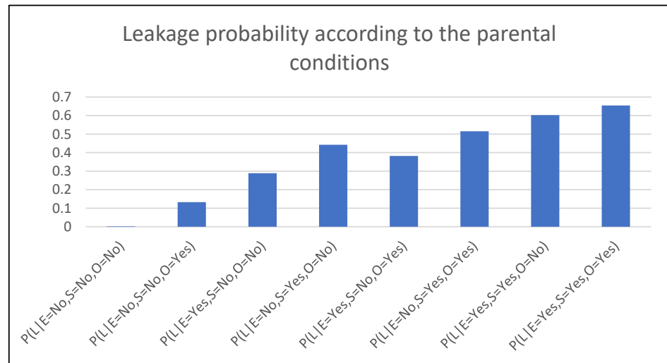
Figure 9. Leakage values with different parent configurations.
