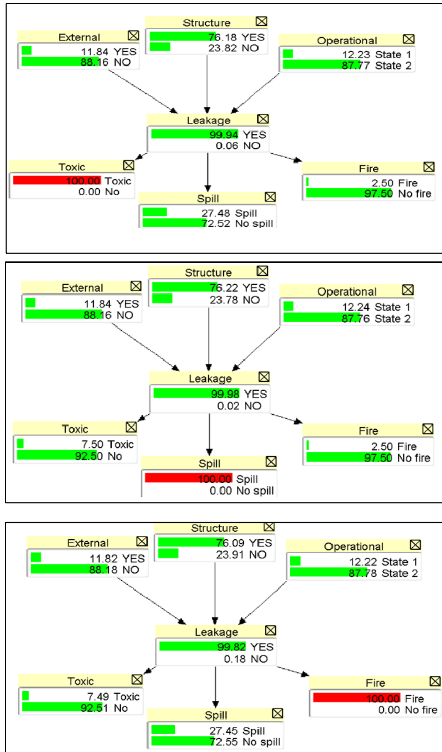
Figure 7. Parent node variations with the child node changes.
