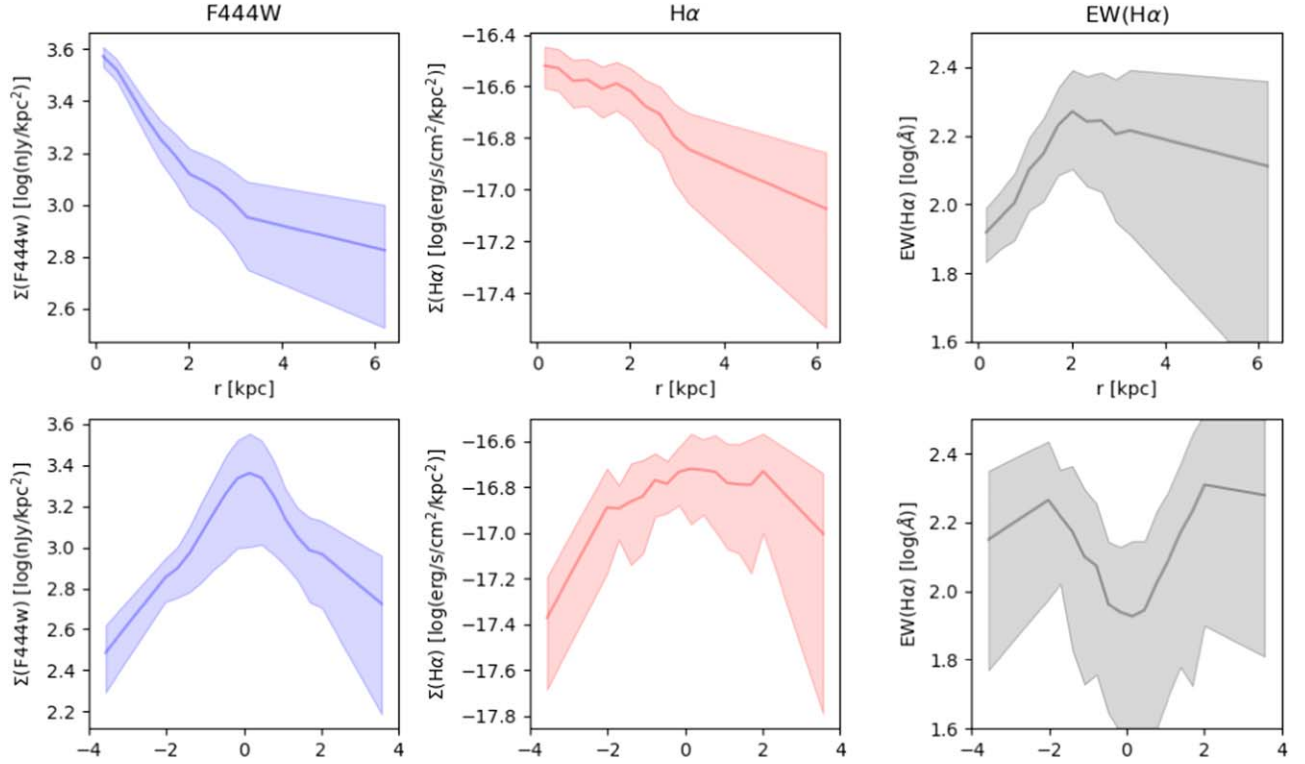
Figure 6. Surface brightness profiles of F444W (left), H \alpha (center), and the radial H \alpha equivalent-width profile (right) made as described in Section 4. The top row shows radially averaged profiles, while the bottom shows the full vertical profile. The H \alpha distribution is much less centrally concentrated than the 4.4 \mu m continuum emission resulting in an H \alpha equivalent-width profile that rises from the center to 2 kpc, consistent with this z = 5.388 galaxy growing inside out in a bulge-disk system.
