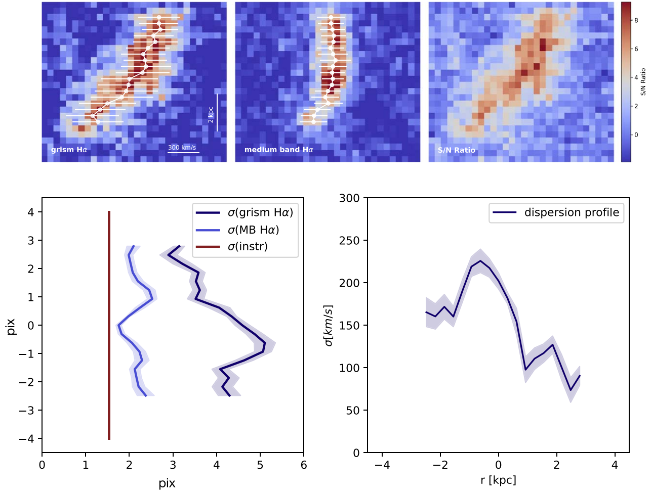
Figure 5. Velocity dispersion profile. As described in Section 3, the width of the H\alpha line in the spectral direction is broadened by three things: the line-of-sight velocity dispersion of the H\alpha gas (including beam smearing), the spectrograph line-spread function, and the intrinsic spatial extent. To measure the line-of-sight velocity dispersion, we subtract the latter two terms off in quadrature. Twister-z5 has a centrally peaked velocity dispersion cospatial with centrally concentrated light, perhaps indicative of a bulge. We measure a disk velocity dispersion of 50\text{--}150\text{ km s}^{-1} , which is likely an upper limit because dynamical forward-modeling has not been performed. The fact that the velocity dispersion peaks in the center and is lower in the disk suggests that the observed velocity gradient is likely due to rotation as opposed to a merger (for which one would expect peaks in the velocity dispersion on either side).
