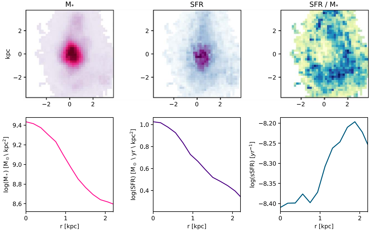
Figure 7. Resolved stellar populations based on SED fitting of the JWST imaging. The top row shows maps of the stellar mass (left), SFR (middle), and specific SFR (right) from spatially resolved SED modeling of the JWST images. The bottom row shows the radial surface density profiles of the stellar mass, SFR, and specific SFR, respectively. A clear central depression can be seen in the specific SFR, a feature that is typically seen in bulge-disk systems growing inside out.
