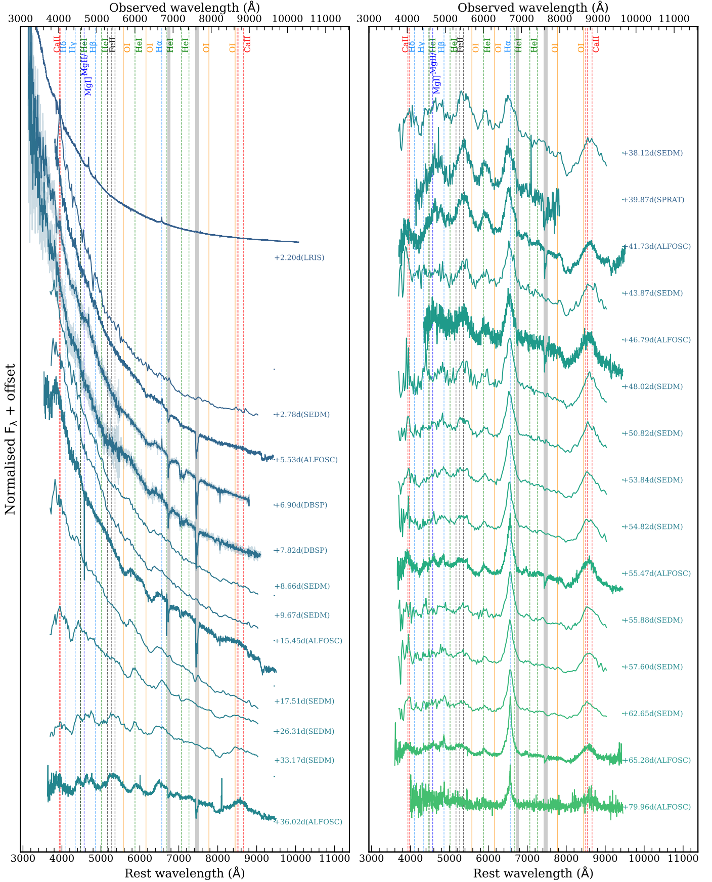
Fig. 3. Spectral series of SN 2022lrg (scaled with the photometry and corrected for MW extinction). Emission lines are marked with vertical dashed lines; throughout the evolution of SN 2022lrg, we detect Balmer lines, He I \lambda 5876 , a broad blend of Fe II ( \sim 5300 \text{\AA} ), and the Ca II NIR triplet. Other marked species are to guide the eye. Telluric features are indicated with grey shaded vertical lines.
