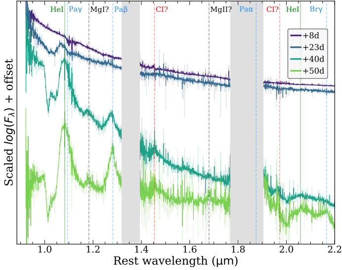
Fig. 15. NIR spectra of SN 2022lxx taken from Tinyanont et al. (2024). The spectra are binned to 5 Å for visual purposes and the original spectra are plotted with lighter colours in the background. The colours of the vertical lines denote the different elements; green is for helium and cyan for hydrogen. The tentatively identified magnesium and carbon are marked with black and red respectively (with a question mark next to the element name). The telluric features are marked with shaded grey regions.
