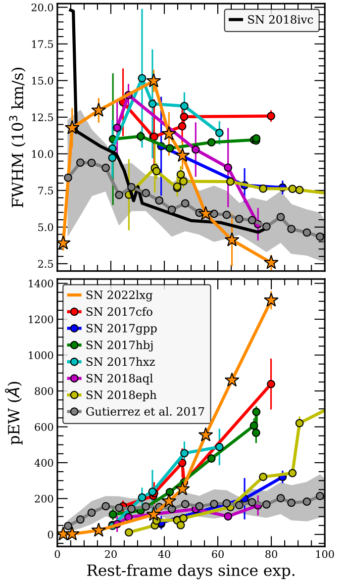
Fig. 14. H\alpha line emission FWHM (top) and pseudo-equivalent width (bottom) compared to other luminous Type II SNe from the P23 sample (adapted from P23). Mean values for regular SNe II from the sample of Gutiérrez et al. (2017) are presented in grey (with the 1\sigma standard deviation plotted as a shaded region). In the top panel, we also plot the H\alpha FWHM of SN 2018ivc (from Bostroem et al. 2020).
