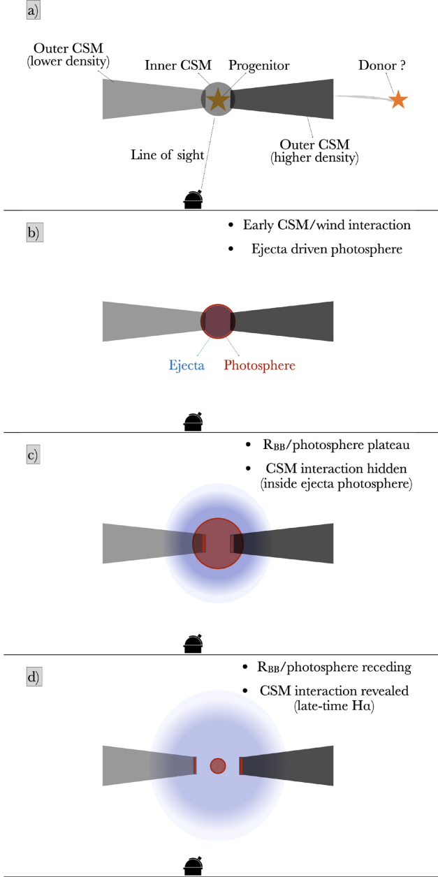
Fig. 22. Example of a possible configuration that gave rise to SN 2022lxx. We envisage a disc-like CSM (with a potentially azimuthally asymmetric density distribution) with the line-of-sight at a low inclination. (a) Before the explosion, we suggest that the CSM closest to the progenitor is denser and could have been formed by material transferred from a donor combined with stellar winds. (b) The fast-moving ejecta crash into the inner dense CSM giving rise to the observed flash-ionisation features and the luminous peak. Within \sim 10 – 15 d this denser CSM is completely swept-up by the ejecta. (c) Between 10 – 35 d, the ejecta encounter the outer, hydrogen-rich, disc-like CSM and encompass it. Broad lines from the free-expanding, cooling ejecta emerge while the radius of the composite photosphere plateaus. (d) After \sim 35 d, the photosphere recedes, the optical depth of the ejecta drops, and the power comes from the interaction. Narrower H\alpha emerges and dominates the spectrum.
