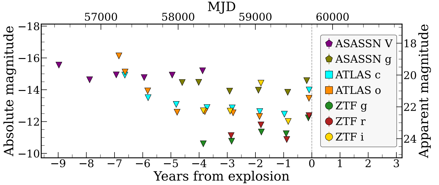
Fig. B.4. Pre-explosion forced photometry at the location of SN 2022lwg from ZTF, ATLAS and ASAS-SN. Individual epochs have been binned per season. Non-detections are shown as downward-facing triangles. The peak time is shown as a dashed vertical line. No significant pre-explosion emission is detected for SN 2022lwg. The forced photometry rules out long-lasting precursors with absolute magnitude M \lesssim -11 mag that might have happened within four years prior to explosion, but before that, they are not deep enough to rule out outbursts similar to those of other SNe.
