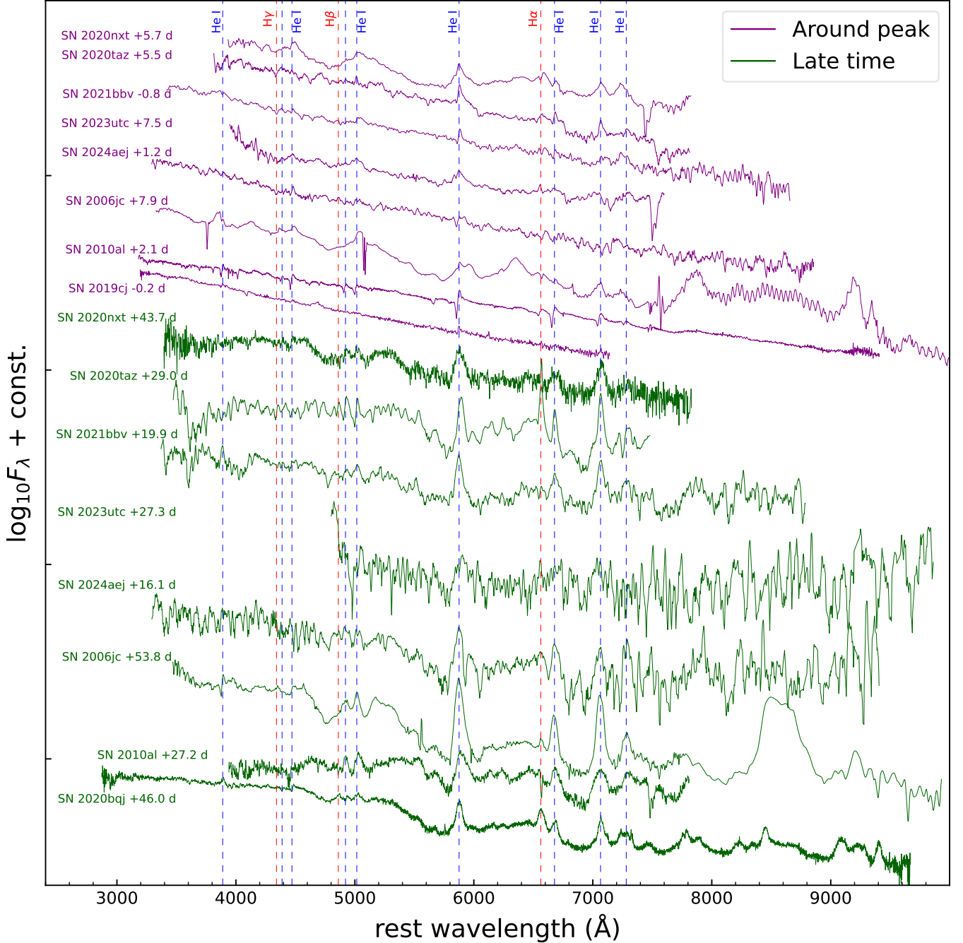
Fig. 14. Comparison of around-peak (purple) and late-time (green) spectra of SNe 2020nxt, 2020taz, 211bbv, 2023utc, and 2024aej with other SNe Ibc at similar phases. All spectra have been corrected for redshift and extinction. Significant He I features are marked by blue dashed lines, while Balmer features by red dashed lines.
