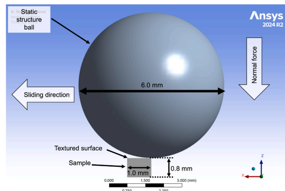
Fig. 3. Finite element analysis (FEA) simulation setup.
