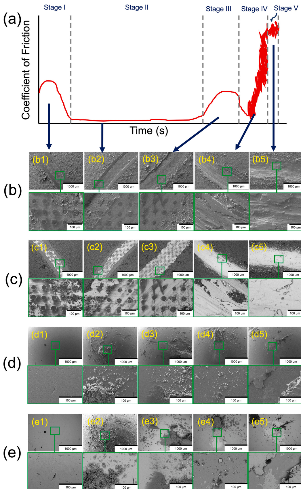
Fig. 11. (a) Schematic drawing of the temporal evolution of COF for the textured surface. (b-e) SEM-(b, d) SE and – (c,e) BSE of the (b-c) worn track and (d-e) counter-body for dimple pattern at 25 % TD according to the stage.
