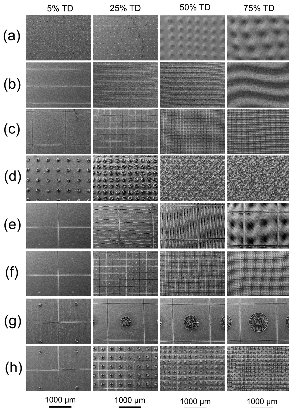
Fig. 5. SEM-SE images of the (a) dimple, (b) groove, (c) grid, (d) concentric ring, (e) dimples-grid, (f) grids-dimple, (g) concentric rings-grid, and (h) grids-concentric ring pattern at 5 %, 25 %, 50 % and, 75 % TD on C28000.
