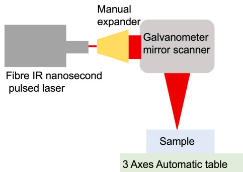
Fig. 1. Schematic drawing of the laser equipment setup.
