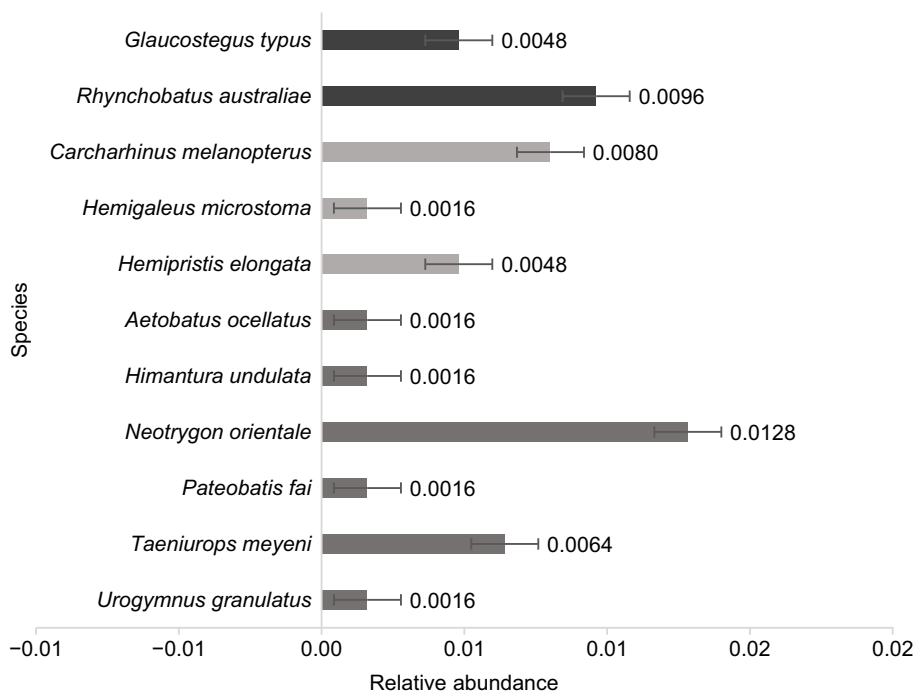
Fig. 3. Composition and relative abundance ( n_{\max} \text{ h}^{-1} ) of target species, including Glaucostegidae, Rhinidae and other elasmobranch species, across all BRUV recordings.
