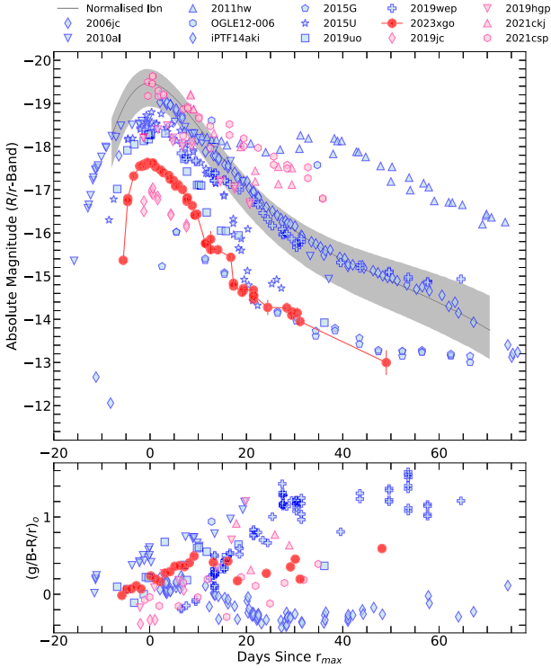
Figure 14. Upper panel of the Figure shows the r -band light curve comparison of SN 2023xgo with a sample of SNe Ibn (blue)(G. Hosseinzadeh et al. 2017). The SN Ibn comparison sample includes SNe 2006jc (R. J. Foley et al. (A. Pastorello et al. 2007; R. J. Foley et al. 2007), 2010al (A. Pastorello et al. 2015a), OGLE-SN-006 (A. Pastorello et al. 2015b), 2011hw (A. Pastorello et al. 2015a), iPTF14aki (G. Hosseinzadeh et al. 2017), 2015U (I. Shivvers et al. 2016; G. Hosseinzadeh et al. 2017), 2015G (G. Hosseinzadeh et al. 2017), 2019uo (A. Gangopadhyay et al. 2020) and 2019wep (A. Gangopadhyay et al. 2022). Phase is plotted in observer-frame days with respect to maxima for all the panels. The SN Icn sample (red) has been taken from D. A. Perley et al. (2022); C. Pellegrino et al. (2022b); T. Nagao et al. (2023). Lower panel shows the colour of SN 2023xgo plotted with the comparison sample.
