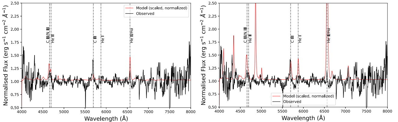
Figure 5. Comparisons of the earliest spectrum having flash ionization signatures of SN 2023xgo with models by I. Boian & J. H. Groh (2019). These are a set of radiative transfer codes (CMFGEN) which generate a set of spectra over different luminosity and mass-loss rates 1 d after explosion. Our spectra are reproduced by spectral model of mass-loss rate 10^{-3} M_{\odot} \text{ yr}^{-1} and increase in flux reproduces the C III \lambda 5696 feature.
