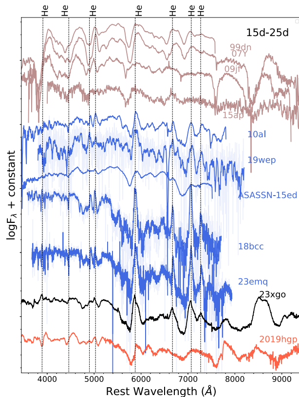
Figure 7. The late epoch (23.48 d) spectral comparison of SN 2023xgo with a group of SNe Ibn (blue), Icn (red), and Ib (brown). SN 2023xgo shows striking similarity with ASASSN-15ed at this phase, with broad P-Cygni features, and is also similar to some SNe Ib.
