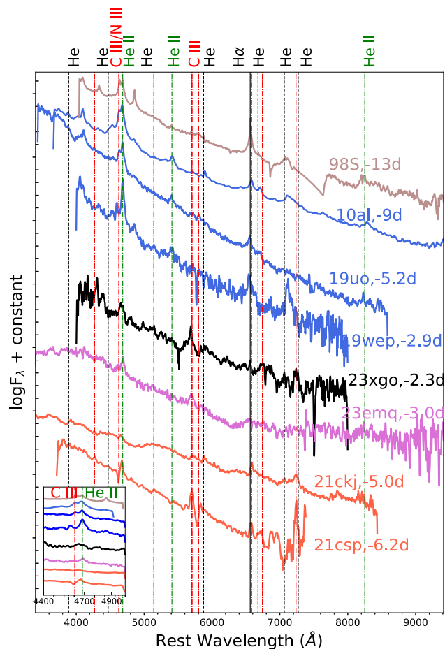
Figure 3. The early spectral comparison of SN 2023xgo (in black) with a selected sample of SNe. The insets mark the unique characteristics of SN 2023xgo, where it shows C III \lambda 5696 as the most prominent feature in the spectral evolution, unlike other SNe Ibn with flash ionization signatures. The different colour coding are: Brown: Type IIn SNe; Blue: Ibn; Red: Icn, and Purple: transitional.
