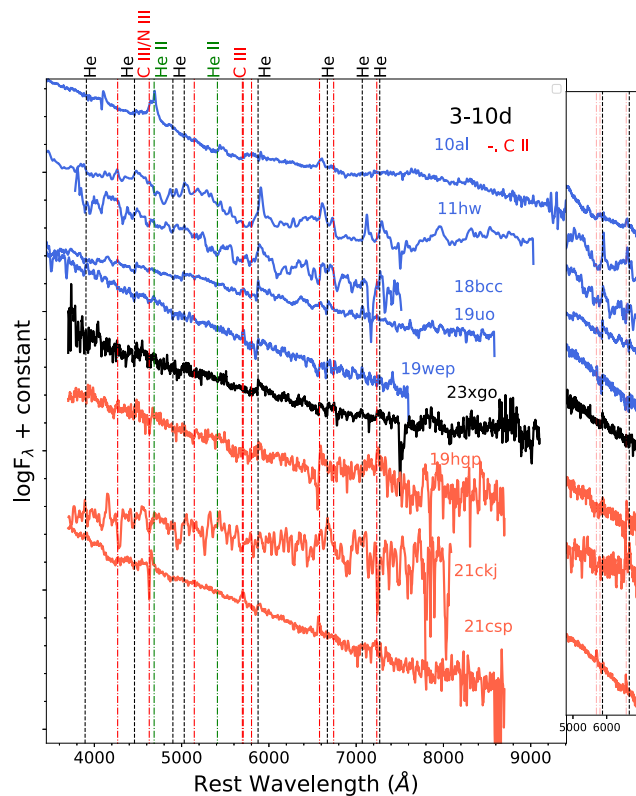
Figure 6. The mid epoch (3 – 10 d) spectral evolution of SN 2023xgo, compared with a set of SNe Ibn (blue) and SNe Icn (red). The right panel of the figure shows the inset region of the 5000 to 6000 Å region where we could detect both the ‘P-Cygni’ and ‘emission’ sub-class of He I \lambda 5876.
