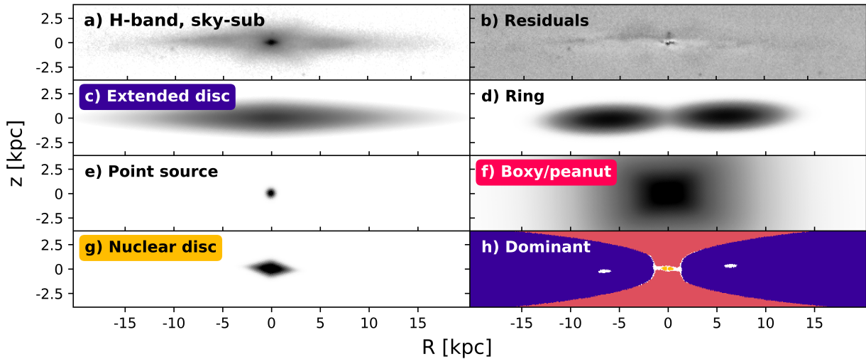
Fig. 1: Components of the image decomposition of PGC 044931. Panel a) is the sky-subtracted, H -band VIRCAM image (arcsinh scaled), b) is the residual map after subtraction of the five components (linear scale), c)–g) are the five components fit with IMFIT (arcsinh scale, limits altered to show maximum structure), and h) shows the spatial extent of the three dominant components. The extended disc is shown in purple, and the boxy/peanut bulge in pink. The nuclear disc (yellow) is very small and only dominates near the centre.
