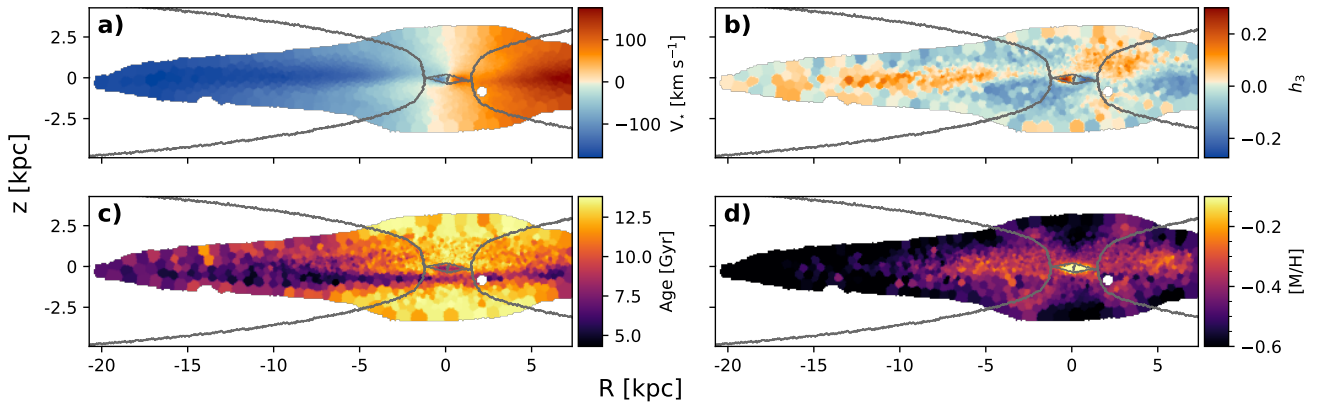
Fig. 2: Masking regions from Figure 1h overlaid as grey contours on light-weighted stellar kinematic (a) V_* , (b) h_3 , and population (c) age, and (d) metallicity maps of PGC 044931. White regions denote masked regions (e.g. due to foreground stars), or areas in which the spaxels did not reach the minimum continuum S/N threshold of 5. A distinctive, metal-rich ‘X’ shape is present in the metallicity map, seen in other galaxies (e.g. NGC 4710; Gonzalez et al. 2016), and in agreement with simulations (e.g. Debattista et al. 2017; Fragkoudi et al. 2020).
