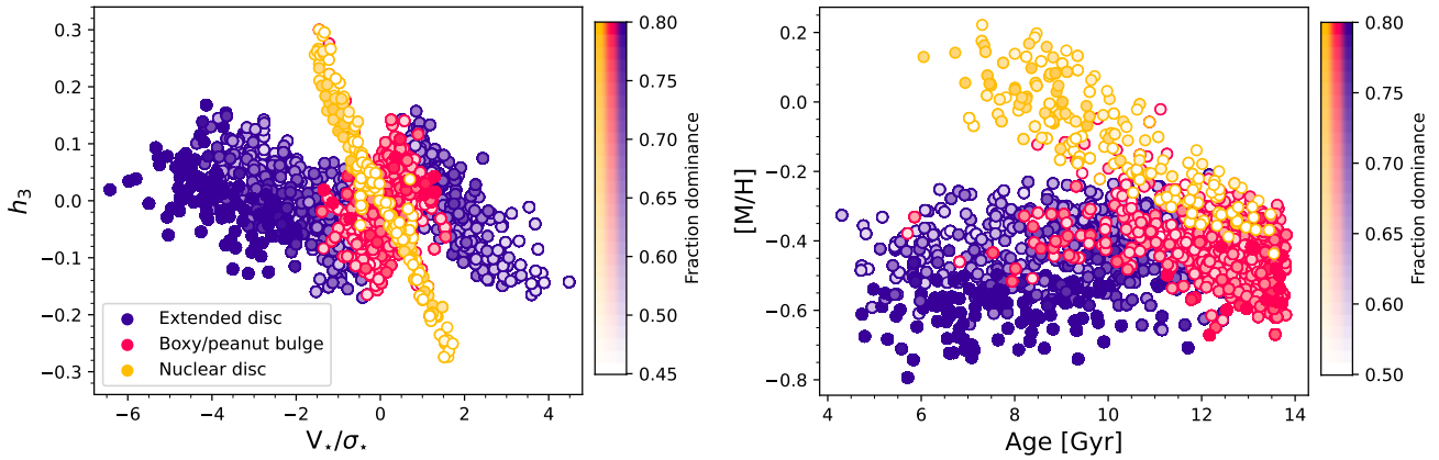
Fig. 3: Separation of the photometric components of PGC 044931 in stellar kinematic and stellar population space. Left: stellar h_3 vs. V_*/\sigma_* , with data points corresponding to Voronoi bins for which the majority of the bin is located in one of the photometric regions. The underlying extended disc, boxy/peanut bulge (bar), and nuclear disc show distinctly different behaviours in this parameter space, allowing us to confidently make inferences about their star formation histories. Right: mean light-weighted stellar metallicity vs. stellar age. The nuclear disc is clearly separated from the bar and boxy/peanut bulge and the boxy/peanut region is on average older and more metal-rich than the underlying disc. The colour saturation indicates the fraction of light attributed to the given component in each bin.
