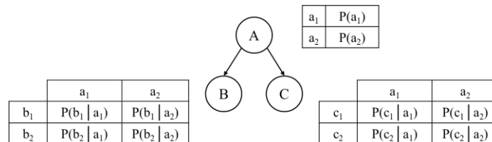
Fig. 2. Example of a Bayesian Network with Conditional Probability Tables.
