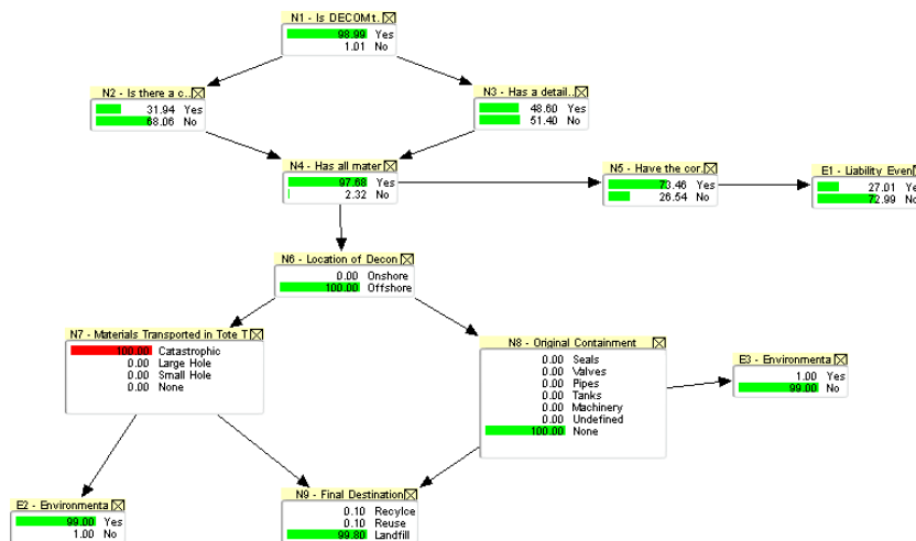
Fig. 10. Test Case 3: Node N7, is set to 100% catastrophic failure.
