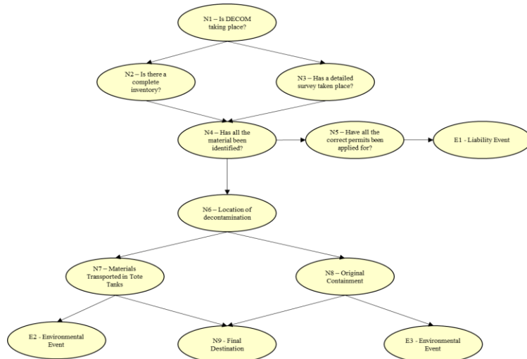
Fig. 4. Bayesian Network
