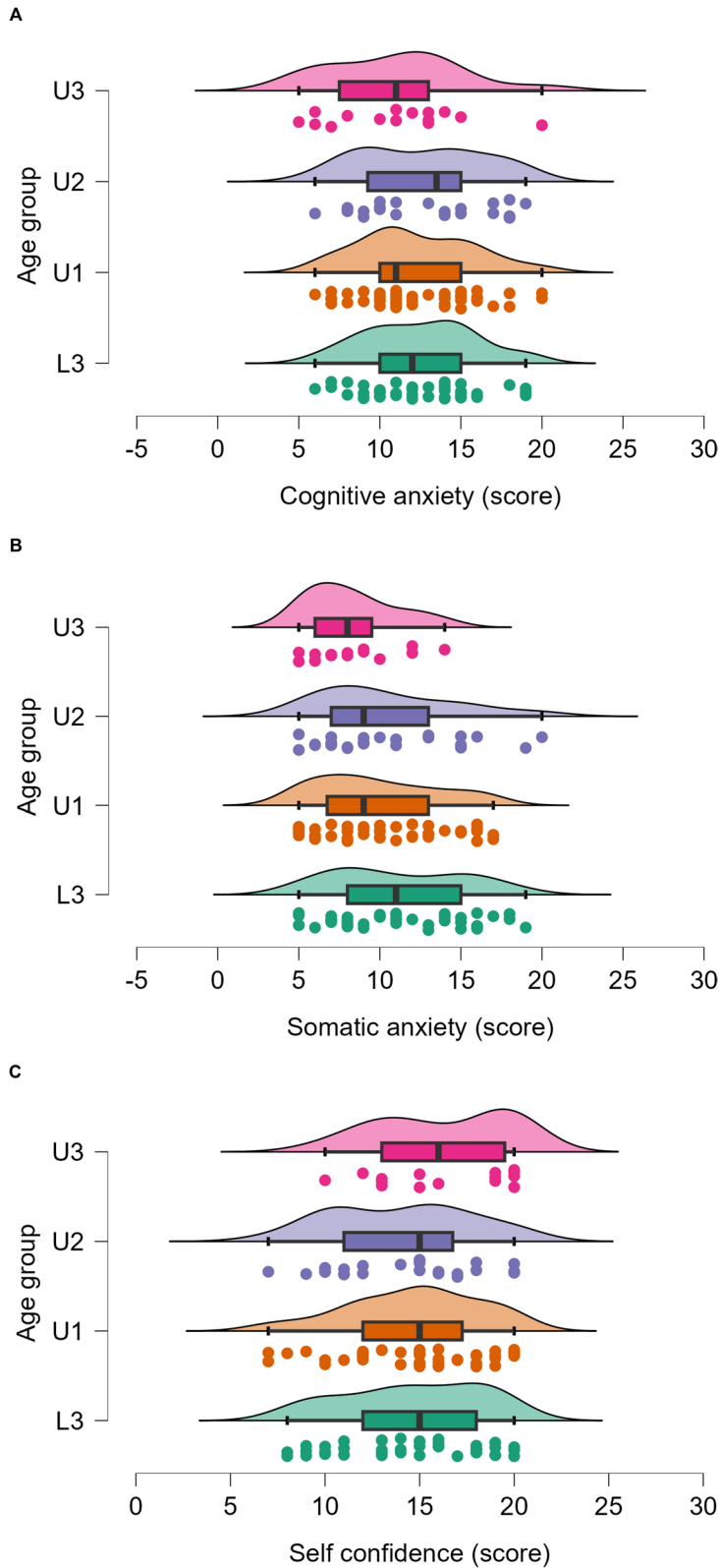
Fig. 1 Raincloud plots of the three CSAI-II constructs across the four age groups. The plot presents a density plot (indicating shape and spread of the data), a boxplot (indicating the median and interquartile range of the data) and the individual raw data points. Panel A Cognitive anxiety; Panel B Somatic anxiety; Panel C Self-confidence. L3 = 15-year olds, U1 = 16-year olds, U2 = 17-year olds, U3 = 18-year olds
