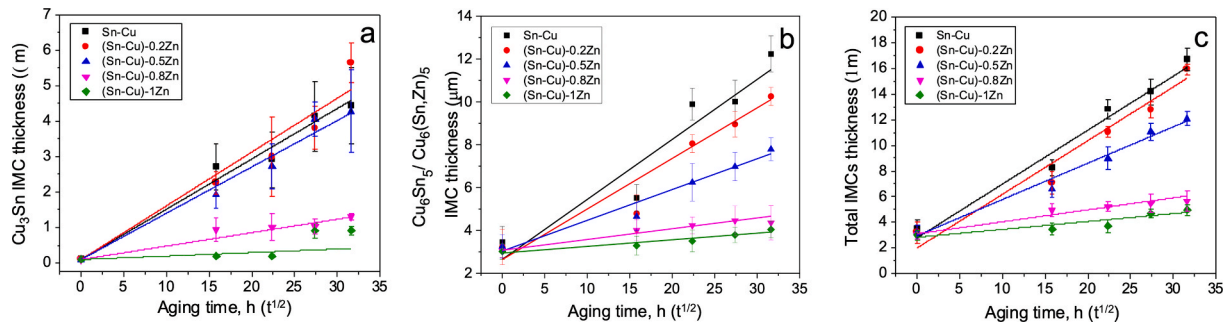
Fig. 6. Evolution of IMC layer thickness with aging time at 150 °C: (a) \epsilon - \text{Cu}_3\text{Sn} , (b) \eta - \text{Cu}_6\text{Sn}_5/\text{Cu}_6(\text{Sn,Zn})_5 , and (c) total IMC thickness. Data points affected by spalling were excluded from the analysis.
