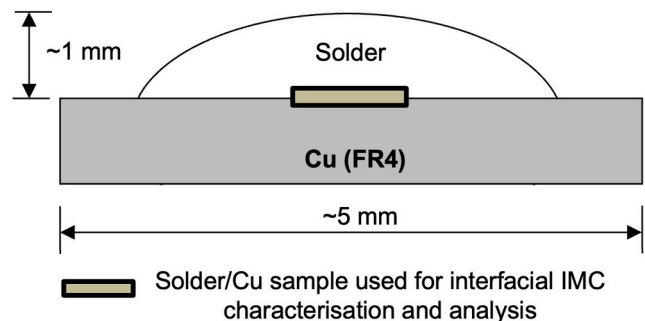
Fig. 1. Schematic cross-sectional geometry of the Sn–0.7Cu/Cu and (Sn–0.7Cu)–Zn/Cu samples.
