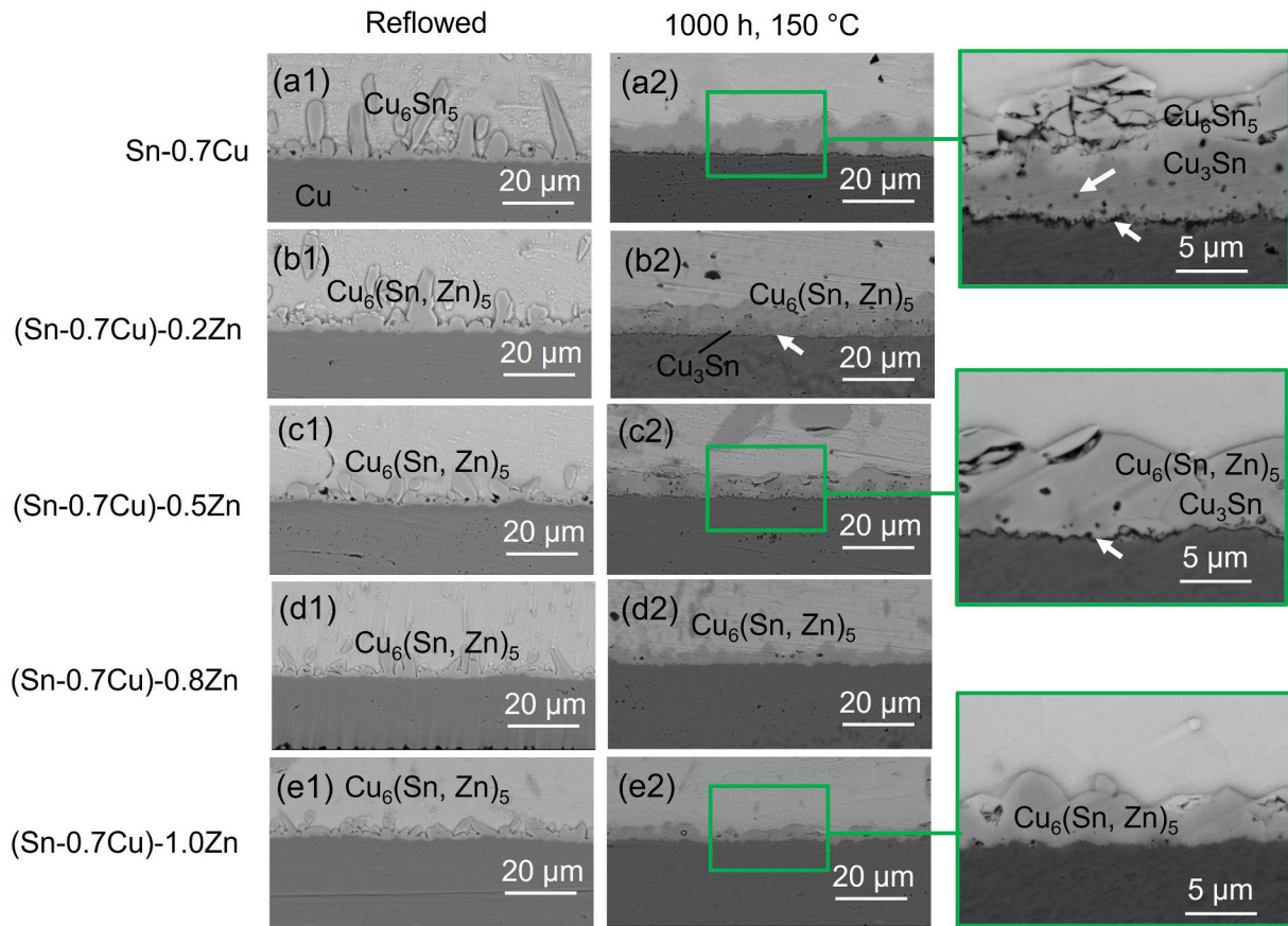
Fig. 5. Cross-sectional microstructure of solder/substrate interfaces for as (a1) –(e1) reflowed and (a2)-(e2) thermally aged (150 °C for 1000 h) samples. Arrows in high magnification image of (a2)–(e2) indicate Kirkendall voids and cracks observed at the interfaces.
