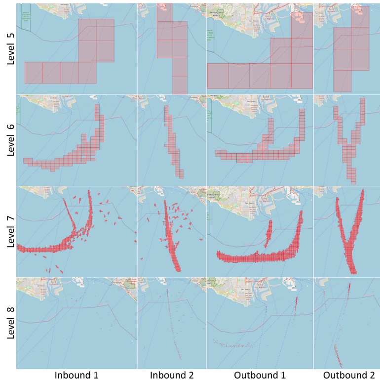
Fig. 11. Inbound/outbound channel extraction using geohash levels 5–8.
