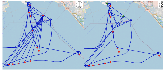
Fig. 2. Comparison of vessel trajectories before and after drift correction. Red points indicate drifted trajectory points, while green points represent the corrected positions. It can be observed that drift events predominantly occur when vessels stop. (For interpretation of the references to colour in this figure legend, the reader is referred to the web version of this article.)
