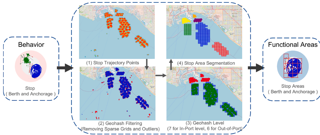
Fig. 5. Workflow for extracting vessel stop functional areas using Geohash filtering and clustering.
