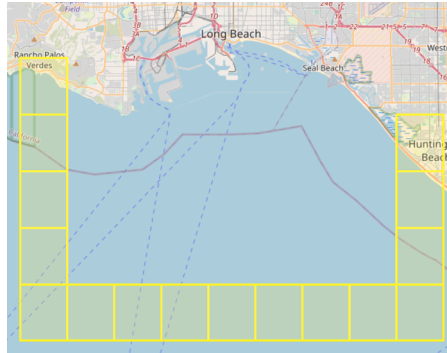
Fig. D.1. Visualization of the boundary of functional areas using level 5 geohash grids. The edge geohash cells are used to identify vessel inbound and outbound points for the corresponding region, supporting the extraction of inbound and outbound trajectories.
