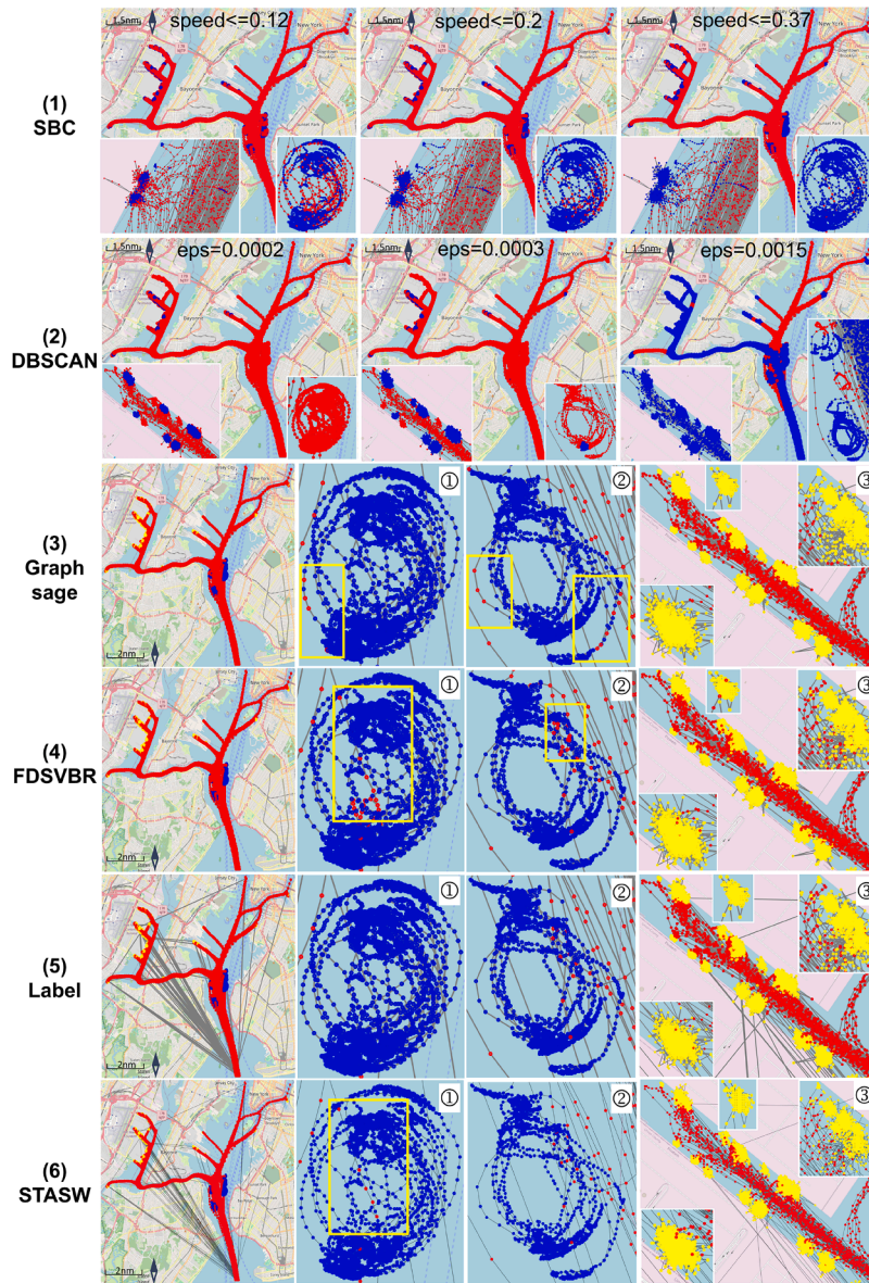
Fig. 13. Visualization of stop behavior recognition by six methods.
