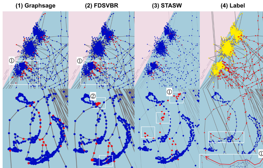
Fig. 14. Visualization of misclassification points for stop recognition.
