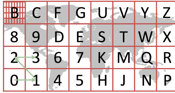
Fig. 3. Illustration of the geohash spatial encoding scheme. The Earth's surface is recursively divided into rectangular cells, each assigned a unique alphanumeric code. Each cell can be further subdivided, with longer codes corresponding to finer spatial resolution.
