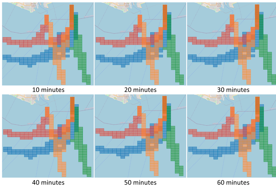
Fig. 9. Extracted inbound/outbound channels under different time-gap thresholds (10–60 mins).
