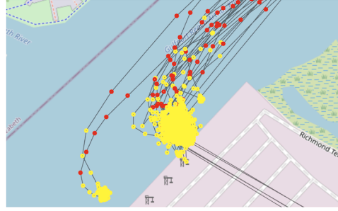
Fig. B.1. Experimental results of stop point recognition without secondary recheck. Red points represent underway trajectories, while yellow points indicate stop points identified by the method. Without rechecking, vessel trajectories immediately before stopping and after leaving are often misclassified as stop points. (For interpretation of the references to colour in this figure legend, the reader is referred to the web version of this article.)
