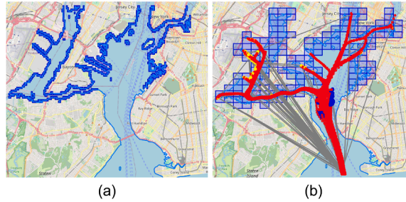
Fig. 4. Geohash encoding of the New York port coastline at level 7 (a) and level 6 (b).
