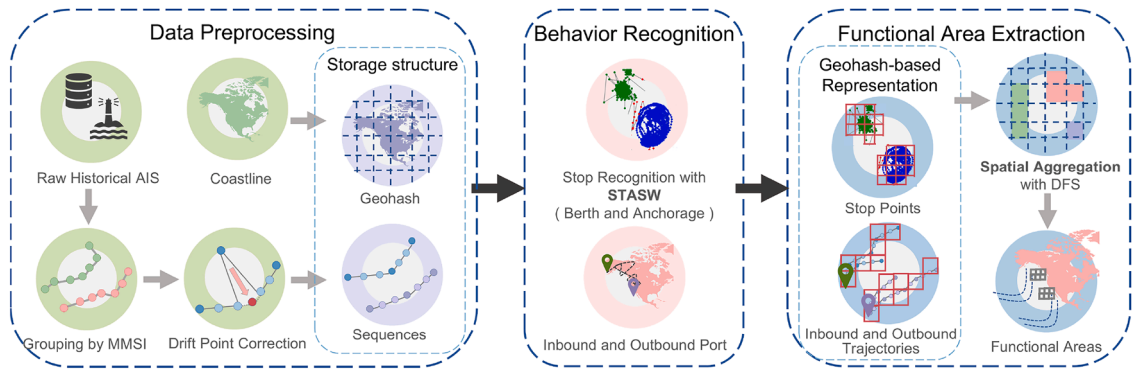
Fig. 1. Overview of the PortMiner framework for unsupervised extraction of port functional areas.
