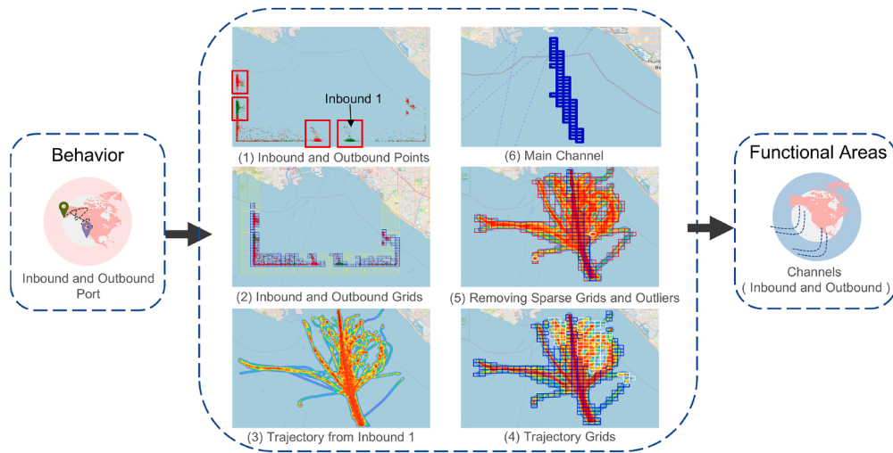
Fig. 6. Workflow for extracting vessel inbound and outbound port channels.
