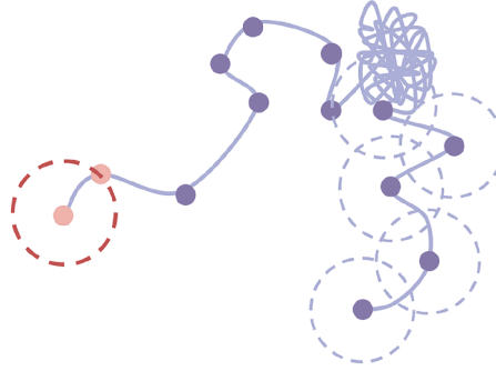
Fig. B.2. Illustration of the second stop point recheck method inspired by DBSCAN. To correct misclassified stop points at the segment boundaries caused by the sliding window approach, points with higher speed and greater distance from the stop cluster (analogous to low-density regions in DBSCAN) are identified and removed. The process checks whether boundary points are core points and stops when a non-core point is found.
