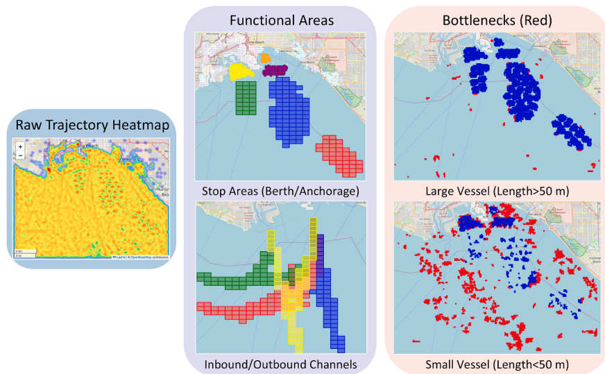
Fig. 25. Diagnostic illustration: raw AIS trajectories versus PortMiner-derived functional structures, including berths, anchorages, channels, and congestion zones.
