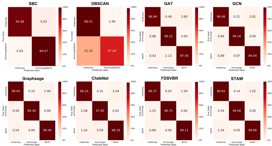
Fig. 12. Confusion matrices for vessel stop behavior recognition across different methods.
