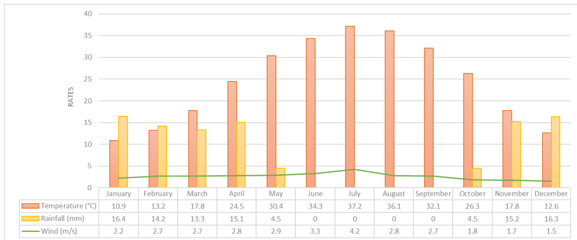
Fig. 6. Temperature, precipitation, and wind speed data for the study area from 1990 to 2020 from the Al-Najaf Climatic Station. Iraq | World Meteorological Organization (wmo. int)
