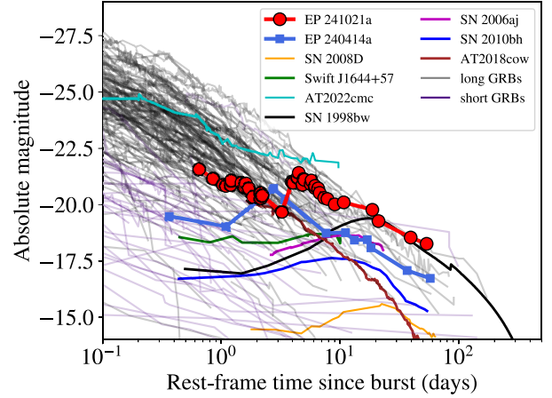
Figure 9. r -band optical light curves of FXT EP241021a (circles) compared to LGRB and SGRB (D. A. Kann, S. Klose & A. Zeh 2006; D. A. Kann et al. 2010, 2011; A. Nicuesa Guelbenzu et al. 2012; D. A. Kann et al. 2024), the SN SBO event XRF 080109/SN 2008D, the X-ray flash source XRF 100316D/SN 2010BH, the LFBOT AT2018cow (D. Xiang et al. 2021), the jetted TDEs AT2022cmc and Swift J1644 + 57 (A. J. Levan et al. 2011; I. Andreoni et al. 2022), and the collapsar FXT EP240414a (J. N. D. Dalen et al. 2025).
