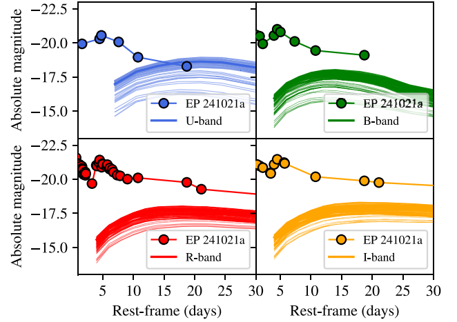
Figure A2. Optical light curves of EP241021a compared to optical thermonuclear transients from hydrodynamic simulation (considering a width range of orientations) of TDEs of WDs from M. MacLeod et al. (2016). The optical light curves remain brighter than the simulations during the whole emission.
