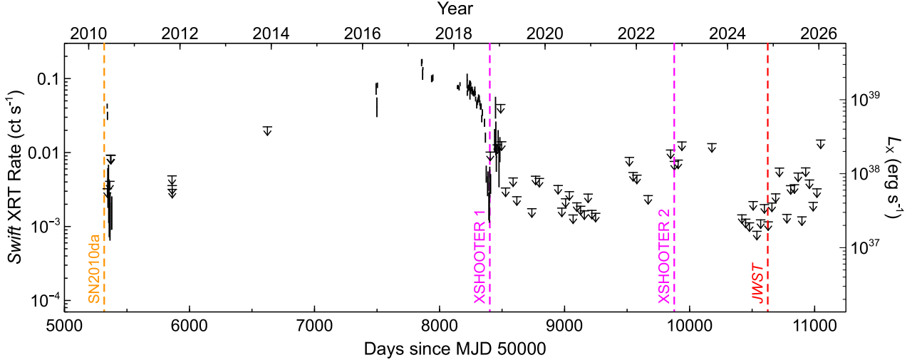
Figure 6. The X-ray lightcurve (0.3–10.0 keV) of ULX-1 from the Neil Gehrels Swift Observatory (Swift; N. Gehrels et al. 2004) following its 2010 outburst. The data have been extracted using the standard online XRT pipeline (P. A. Evans et al. 2009). During the main period of activity (prior to MJD 58500) the data are shown on a per-observation basis, while after this date we extract the XRT data using \sim month-long bins to better showcase the limits on continued activity placed by Swift; where only upper limits on the brightness can be placed, these are computed at the 2\sigma level. In addition to showing the evolution of the X-ray luminosity, we also indicate the date of the SN2010da event (that we take to mark the onset of the outburst) and the dates on which optical/IR spectra were taken with vertical dashed lines.
