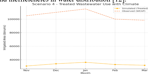
Figure 8. Scenario 4 – Monthly Irrigation Using Treated Water (Climate &amp; WEAP)
