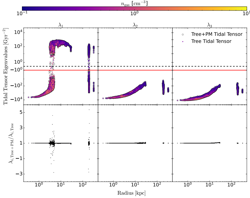
Fig. B.3: Star forming gas tidal tensor eigenvalues distribution at z = 0 , for the halo 6. Top : Distribution for the fiducial variation at lower resolution with/without including the tidal tensor from long-range gravity contributions. Bottom : Ratio of the eigenvalues for the two different calculations of the tidal tensor.
