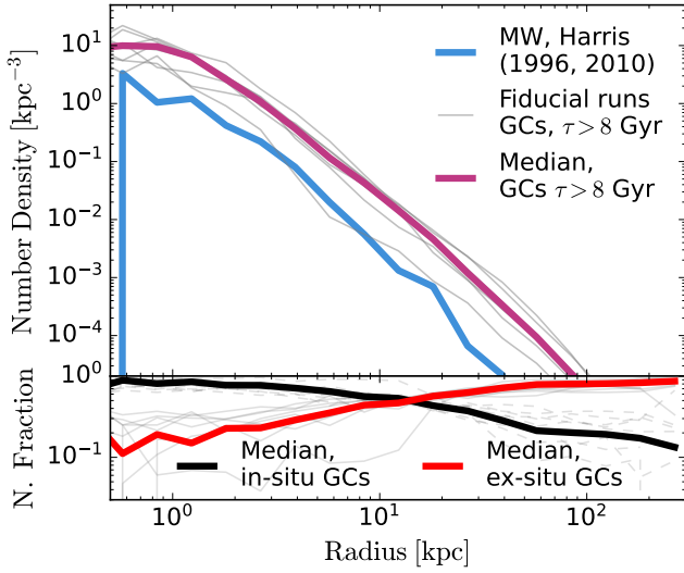
Fig. 12. Top: number density radial profile of the old ( \tau > 8 Gyr) simulated GCs of the fiducial runs, in gray, in comparison to the distribution of GCs in the MW. Bottom: fraction of in situ (dashed gray lines) and ex situ (continuous gray lines) GC candidates at the same age cut as a function of the galactocentric radius.
