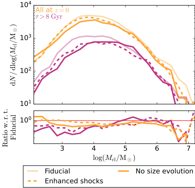
Fig. 6. Top: Halo 6 all SCs MFs for the enhanced shocks (boosting tidal shocks by a factor of 10) and for the no size evolution (without evolving the clusters half-mass radius) variations in comparison to the fiducial model (see Table 1). The colours correspond to MFs at different age cuts, as described in the top left corner of the figure. Bottom: ratio of the MFs with respect to the correspondent MF from the fiducial model.
