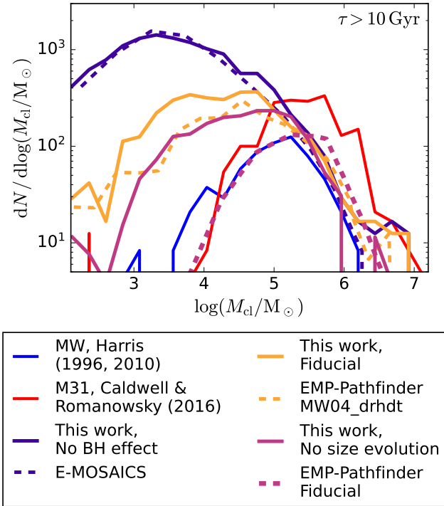
Fig. 14. Comparison of this work simulated MFs with respect to those of E-MOSAICS (Pfeffer et al. 2018; Kruijssen et al. 2019a) and EMP-Pathfinder (Reina-Campos et al. 2022a, 2023) projects. All the simulated MFs correspond to old SCs at the \tau > 10 Gyr age cut. From our work, we only plot the models that compare well to the mentioned projects. For E-MOSAICS, the distribution corresponds to the median MF of 25 zoom-in MW-mass simulations plotted in Fig. 8 in Reina-Campos et al. (2022a). From the same figure, we extracted the fiducial MF of EMP-Pathfinder (with no size evolution) while the MW04_drhd model, that includes size evolution, was extracted from Fig. 4 in Reina-Campos et al. (2023).
