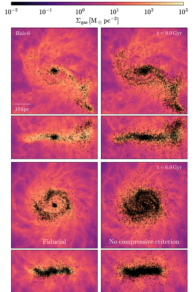
Fig. 5. Face-on and edge-on gas surface density projections of halo 6 at 9 Gyr (top) and 6 Gyr (bottom) of lookback time for two different model choices for SCs formation. The location of newly formed SCs, i.e. \tau \lesssim 200 Myr, is highlighted with black crosses. Left: Fiducial model with SCs forming only in tidally compressive gas. Right: no compressive criterion where SCs formation is not constrained to these environments only.
