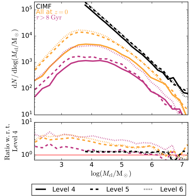
Fig. 7. Top: Halo 6 all SCs MFs for the fiducial run at three resolution levels: level 4, level 5, and level 6. The colours correspond to MFs at different age cuts, as described in the top left corner of the figure. Bottom: ratio of the MFs with respect to the correspondent MF at level 4.
