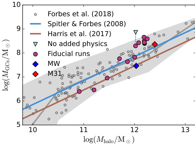
Fig. 13. GC system-mass-to-halo-mass relation for the simulated halos, including a compilation of galaxies across different masses and morphologies presented in Forbes et al. (2018), and the MW and M31 systems from the values quoted in Table 2. The gray continuous line is the median and the shaded region is the 2\sigma of the distribution of the galaxies in Forbes et al. (2018). Also included are the empirical relations derived by Spitler & Forbes (2009); Harris et al. (2017). For the fiducial model, the simulated GC systems masses, according to the GC candidate selection and old ages ( \tau > 8 Gyr), generally lie inside the observed scatter of the empirical relation. The no added physics variation of halo 6, on the other hand, gives a total mass in old GCs that sits above the observational scatter and almost an order of magnitude higher than the fiducial model.
