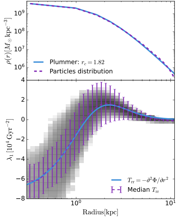
Fig. B.1: Tidal tensor from a simulated Plummer sphere. Top : Profile fit of the simulated sphere. Bottom : Distribution of the highest tidal tensor eigenvalue, as calculated in the simulation compared to the analytical eigenvalue.
