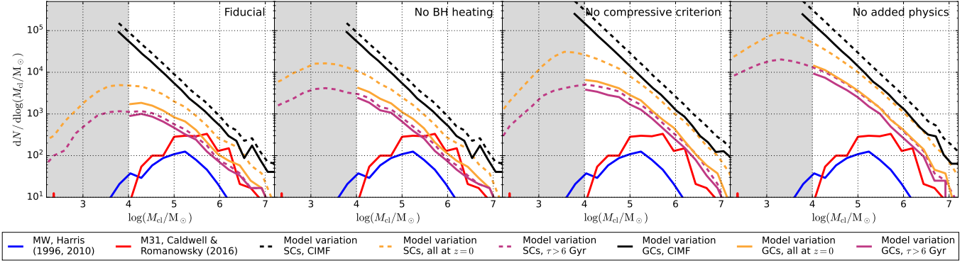
Fig. 4. Halo 6 cluster mass functions for the variations of the star cluster model choices (see Table 1). From left to right, the cluster mass functions for: fiducial model with all the physics described in Sect. 2.2, no BH heating variation of the SCs evolution, no compressive criterion variation of the SCs formation, and the no added physics base model. The MFs for all SCs and for the GC selection (see Sect. 3.2) are included for all the model variations, as well as the CIMFs. For comparison, the observed GCMFs from the MW and M31 are included (as obtained from Harris 1996, 2010; Caldwell & Romanowsky 2016). The shaded region in all the panels denotes the SC mass range that is excluded in our GC selection.
