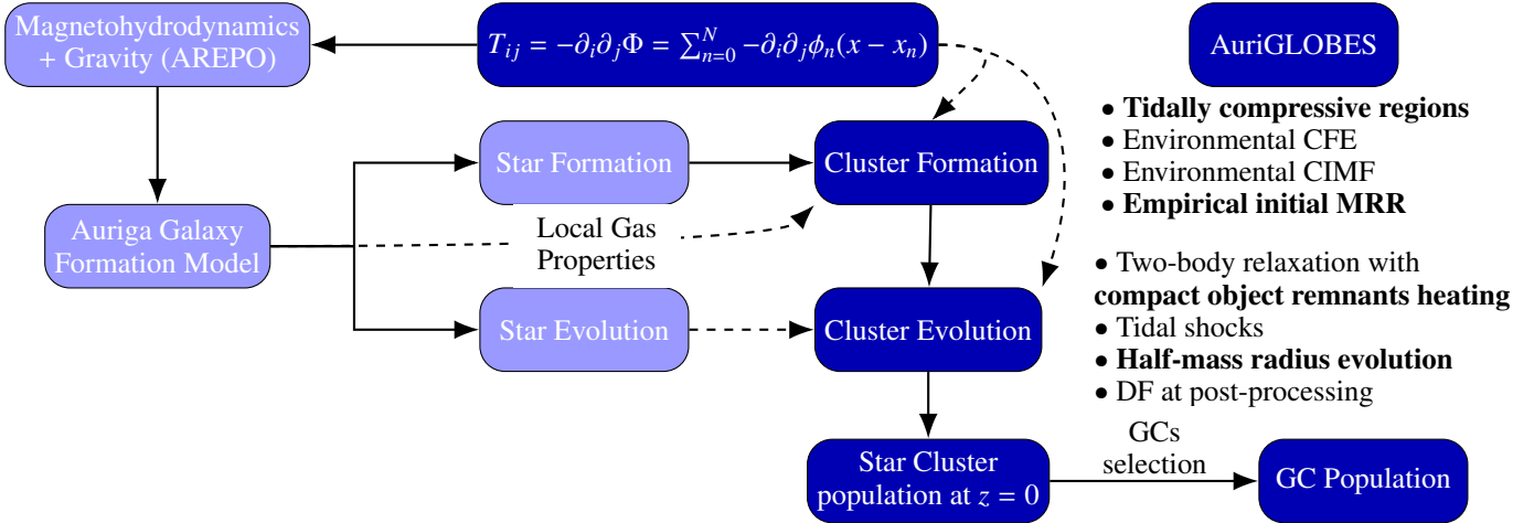
Fig. 1. The AuriGLOBES star cluster formation and evolution model. The base simulation code and the Auriga galaxy formation model, with star formation and evolution stages, are depicted in the light blue boxes. The AuriGLOBES extension to the base simulation is depicted in the dark blue boxes. Continuous arrows represent a direct relation, while dashed arrows represent a dependency relation. Bold fonts highlight extensions with respect to previous models. The used acronyms are: cluster formation efficiency (CFE), cluster initial mass function (CIMF), mass radius relation (MRR), dynamical friction (DF), and globular clusters (GCs).
