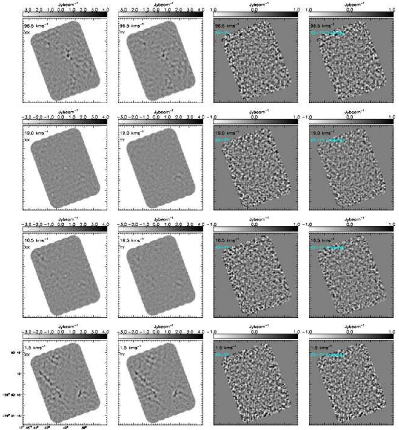
Fig. 6. Left to right columns show the XX, YY, XX - YY, and XX - a^{\text{Cl}}(v)YY synthesized intensity maps of selected velocity channels. These images were generated using the 12m-Array data only (Section 2), and were further tapered by a Gaussian weighting function of FWHM = 1''.5 . The Cl line emission close to v_{\text{LSR}} \sim 20 \text{ km s}^{-1} is subject to foreground absorption, such that the images are dominated by the point-like absorption signature against Sgr A*. Extended Cl emission features surrounding Sgr A* are present away from v_{\text{LSR}} \sim 20 \text{ km s}^{-1} .
