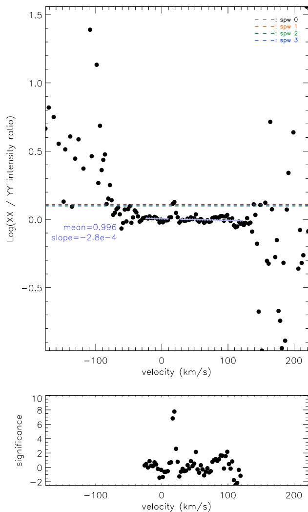
Fig. 5. Top panel shows the derived intensity ratio between the XX and the YY correlations ( F_{XX}^{Cl}(v)/F_{YY}^{Cl}(v) ) from C1 line velocity channel synthesized image, as a function of v_{lsr} . We overplotted the XX and YY intensity ratios derived from the continuum data of the inner 7 12m-Array mosaic fields (dashed lines, color coding the four spectral windows). The large scattering in the redshifted and blueshifted ends are because we did not detect C1 emission or absorption and therefore fittings of F_{XX}^{Cl}(v)/F_{YY}^{Cl}(v) did not converge. We performed linear regression for the high S/N spectral channels, and derived the \pm 1 standard deviation ( \sigma_v^{Cl} ) of the differences from the regression line. Results of linear regression is shown by light blue symbols. We plot (F_{XX}^{Cl}(v)/F_{YY}^{Cl}(v)) / (\sigma_v^{Cl}) in the bottom panel.
