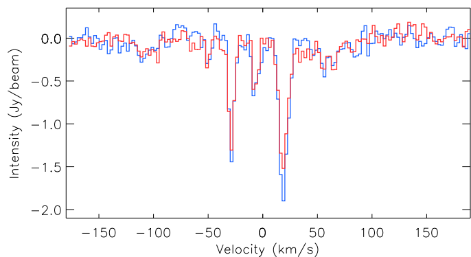
Fig. 7. The C1 line spectra taken from a single synthesized beam area surrounding the Sgr A*. Blue and red lines present the XX and YY polarizations.
