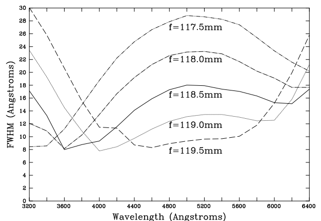
Figure 8. Calculated Full Width Half Maximum as a function of focus distance ( f ) from the last surface of the camera lens to the detector and assuming 1.0 arcsec seeing. The calculation has been carried out at the nominal focus ( f=118.5\text{mm} ) and values of \pm 0.5\text{-} and \pm 1.0\text{-mm} either side.
