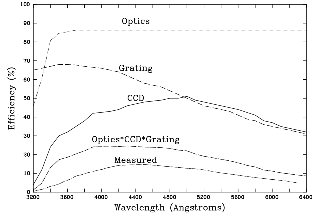
Figure 2. CCD quantum efficiency (solid line), grating throughput (dashed line) as a function of wavelength and optical throughput (dotted line). The product of the three is shown as a dot-dash line as is a prediction of the overall spectrograph throughput. The throughput measured from observations of spectrophotometric standards is shown as a dot-dot-dash line (See section 5.2).
